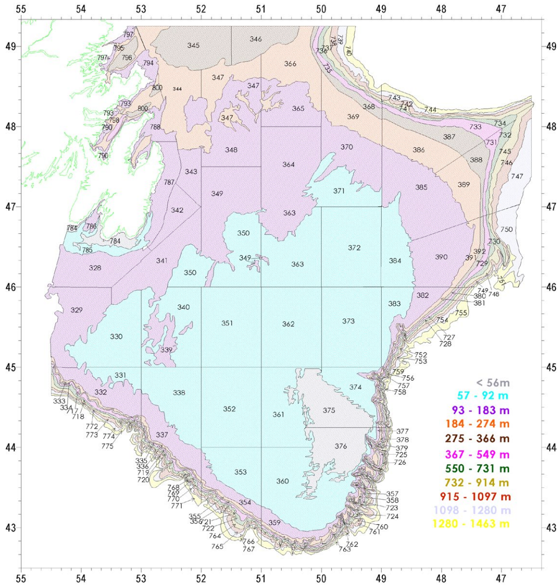
Figure 1. Designation of strata in NAFO divisions 3LNO.
