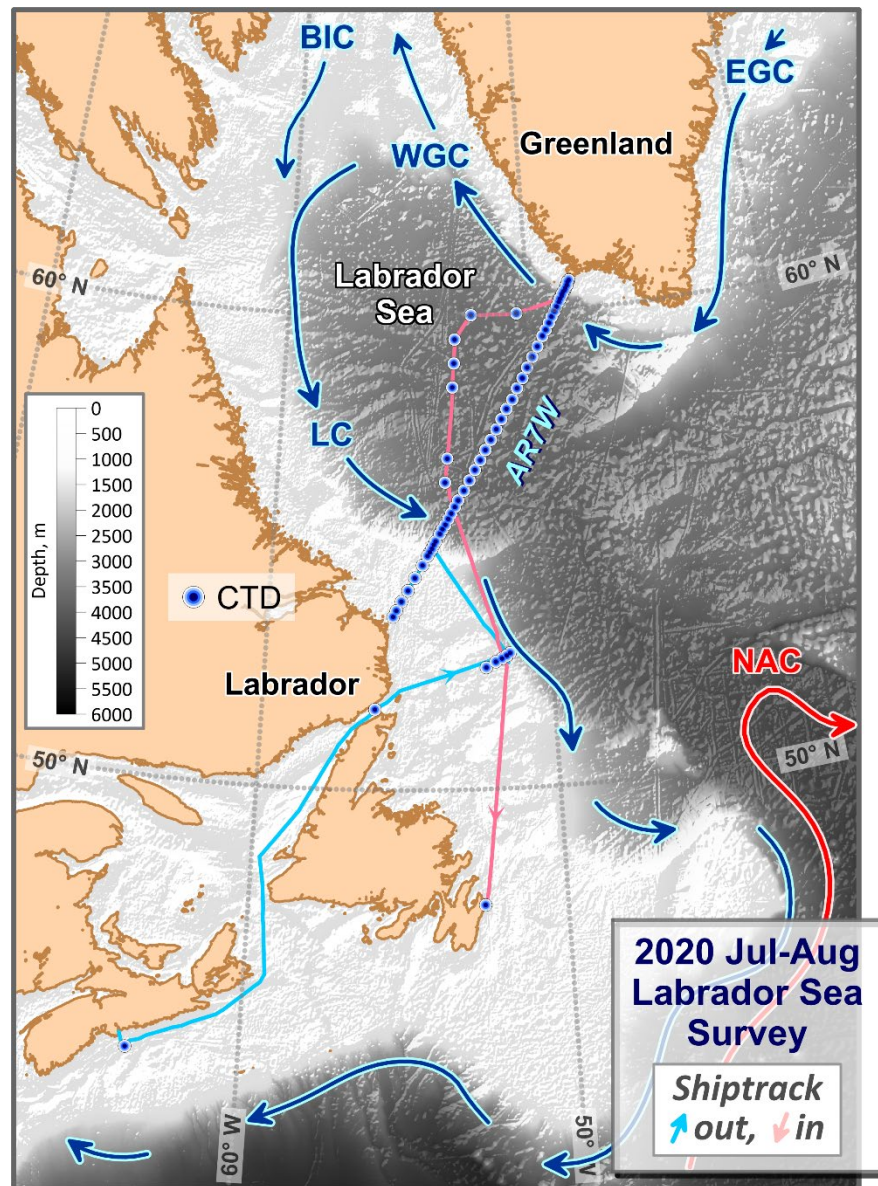
Figure 1. (a) Topography and major deep-water currents in the Labrador Sea and adjacent regions of the North Atlantic. The 2020 July-August Labrador Sea mission CTD stations.
