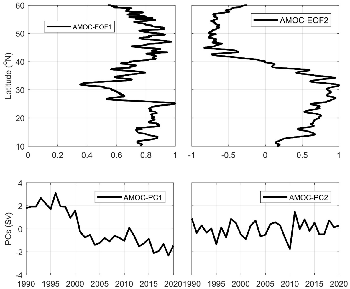
Figure 20. EOF patterns of AMOC (top panel) and associated PCs of these EOFs (bottom panel).
