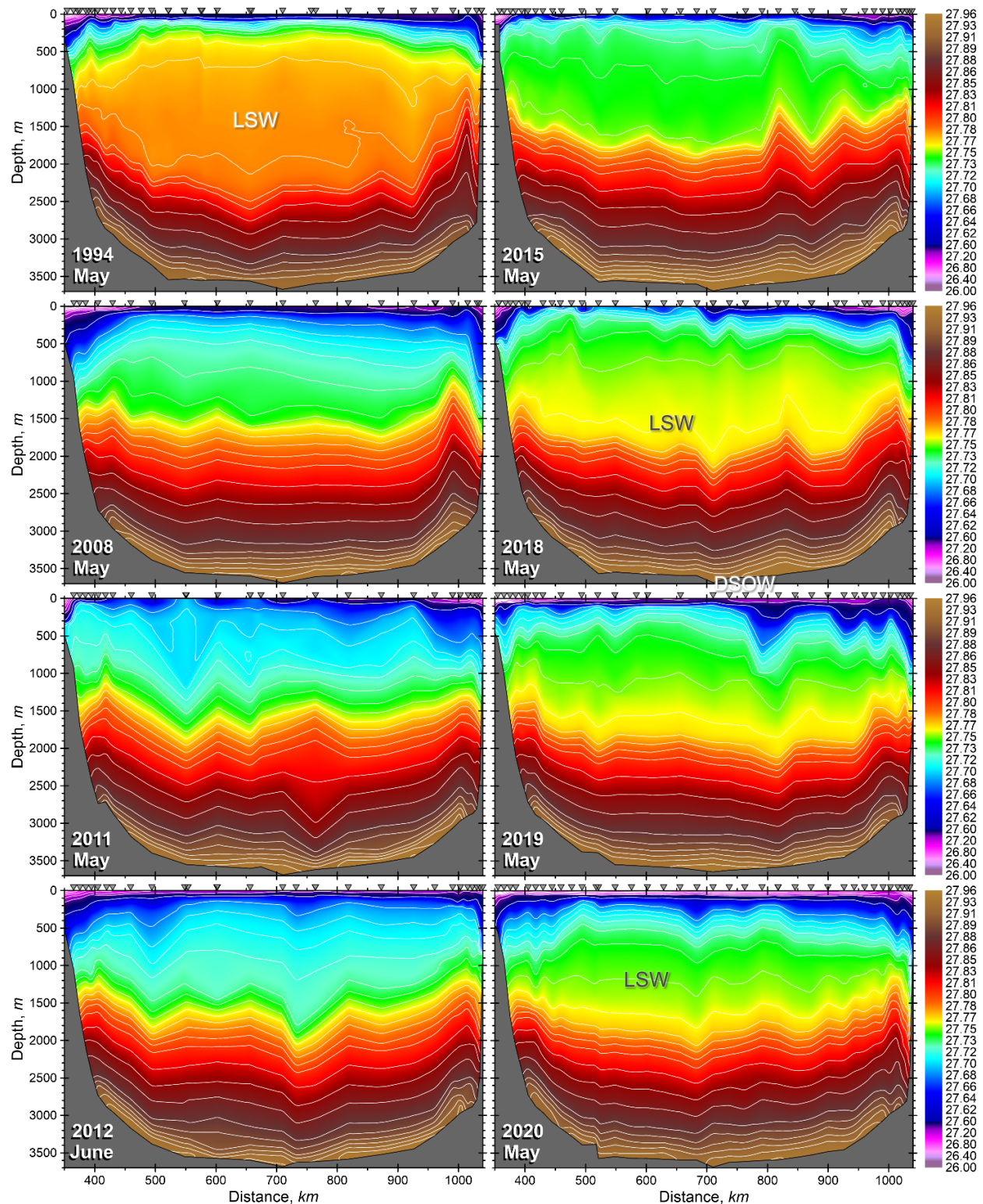
Figure 14. Distributions of potential density (referenced to the sea surface, \text{kg/m}^3 ) on the AR7W line across the Labrador Sea from annual spring-summer surveys in 1994, 2008, 2011, 2012, 2015, 2018, 2019 and 2020. Inverted triangles indicate station locations. LSW, NEADW and DSOW indicate Labrador Sea Water, Northeast Atlantic Deep Water and Denmark Strait Overflow Water, respectively.
