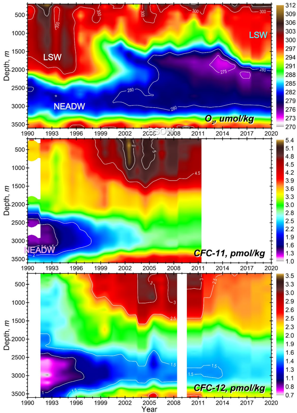
Figure 9. Annual composite profiles of dissolved oxygen (upper panel), CFC-11 (middle panel) and CFC-12 (lower panel) in the central region of the Labrador Sea (time period: 1990-2019, depth range: 200-3500 m). LSW, NEADW and DSOW indicate Labrador Sea Water, Northeast Atlantic Deep Water and Denmark Strait Overflow Water, respectively. Thorough quality control and time-dependent corrections, based on multivariate analysis of oceanographic data (e.g., in near-stagnant or slow-evolving water mass layers such as the NEADW core) were applied to the data sets before averaging.
