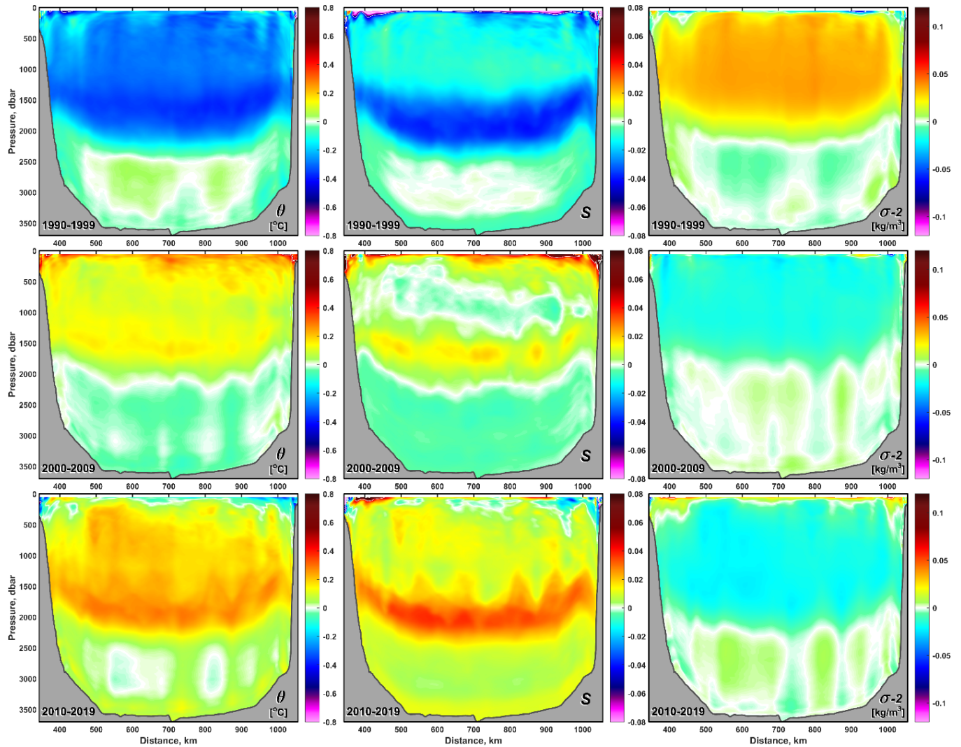
Figure 16. Average decadal 1990-1999 (upper row), 2000-2009 (middle row) and 2010-2019 (lower row) anomalies of temperature (left column), salinity (central column) and density (right column) on the AR7W line, based on the entire collection of both Canadian and international Labrador Sea oceanographic survey data. The decadal anomalies are based on averaging of annual anomalies referenced to the 1990-2020 climatological normal presented in Figure 15.
