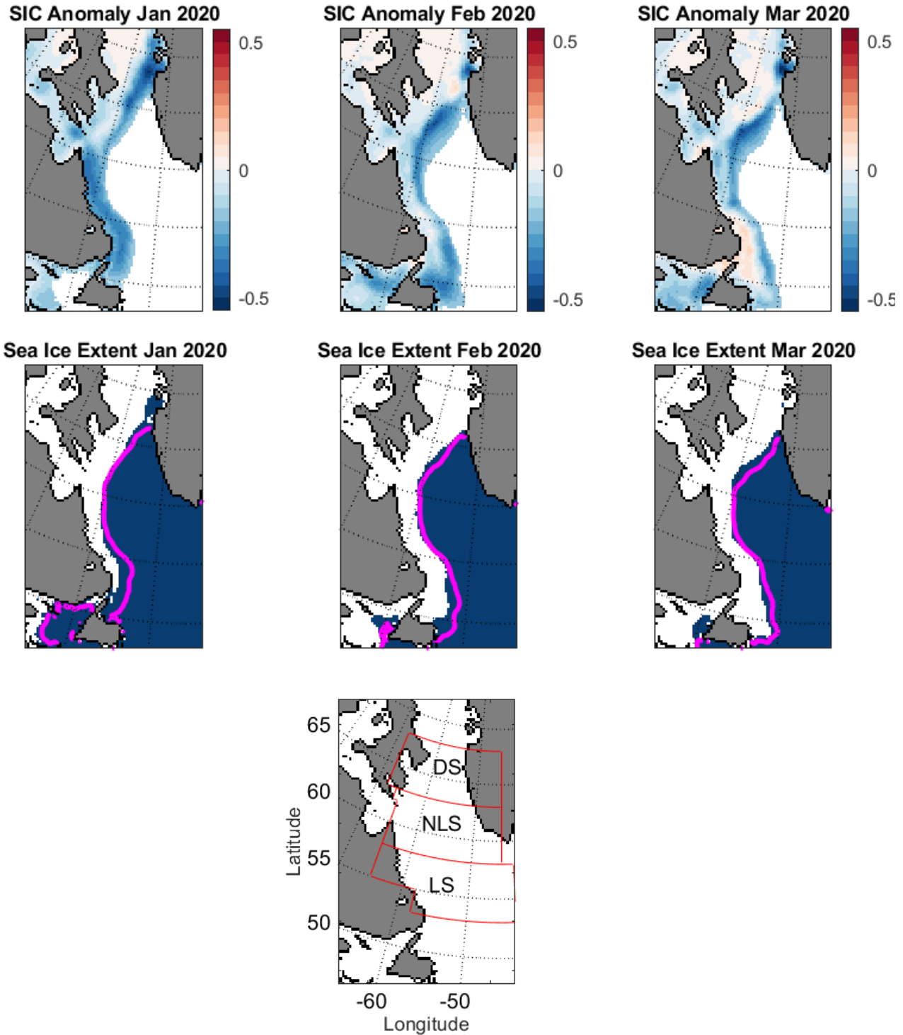
Figure 7. Sea ice concentration anomalies (top) and sea ice extent (middle) for January-March 2020 as derived by the US National Snow and Ice Data Center (reference period 1979-2000) http://nsidc.org/ . The magenta lines show the median ice edge for 1981-2010. Davis Strait (DS), Northern Labrador Sea (NLS), and Labrador Shelf (LS) regions (bottom panel).
