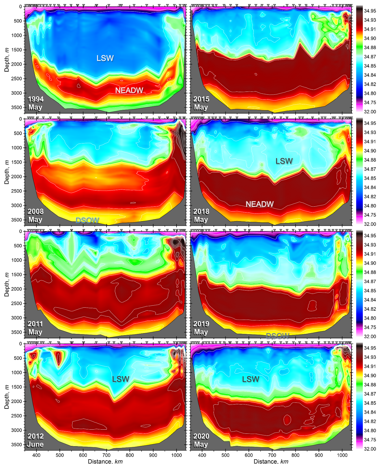
Figure 13. Distributions of salinity on the AR7W line across the Labrador Sea from annual spring-summer surveys in 1994, 2008, 2011, 2012, 2015, 2018, 2019 and 2020. Inverted triangles along the top of each panel indicate station locations. LSW, NEADW and DSOW indicate Labrador Sea Water, Northeast Atlantic Deep Water and Denmark Strait Overflow Water, respectively.
