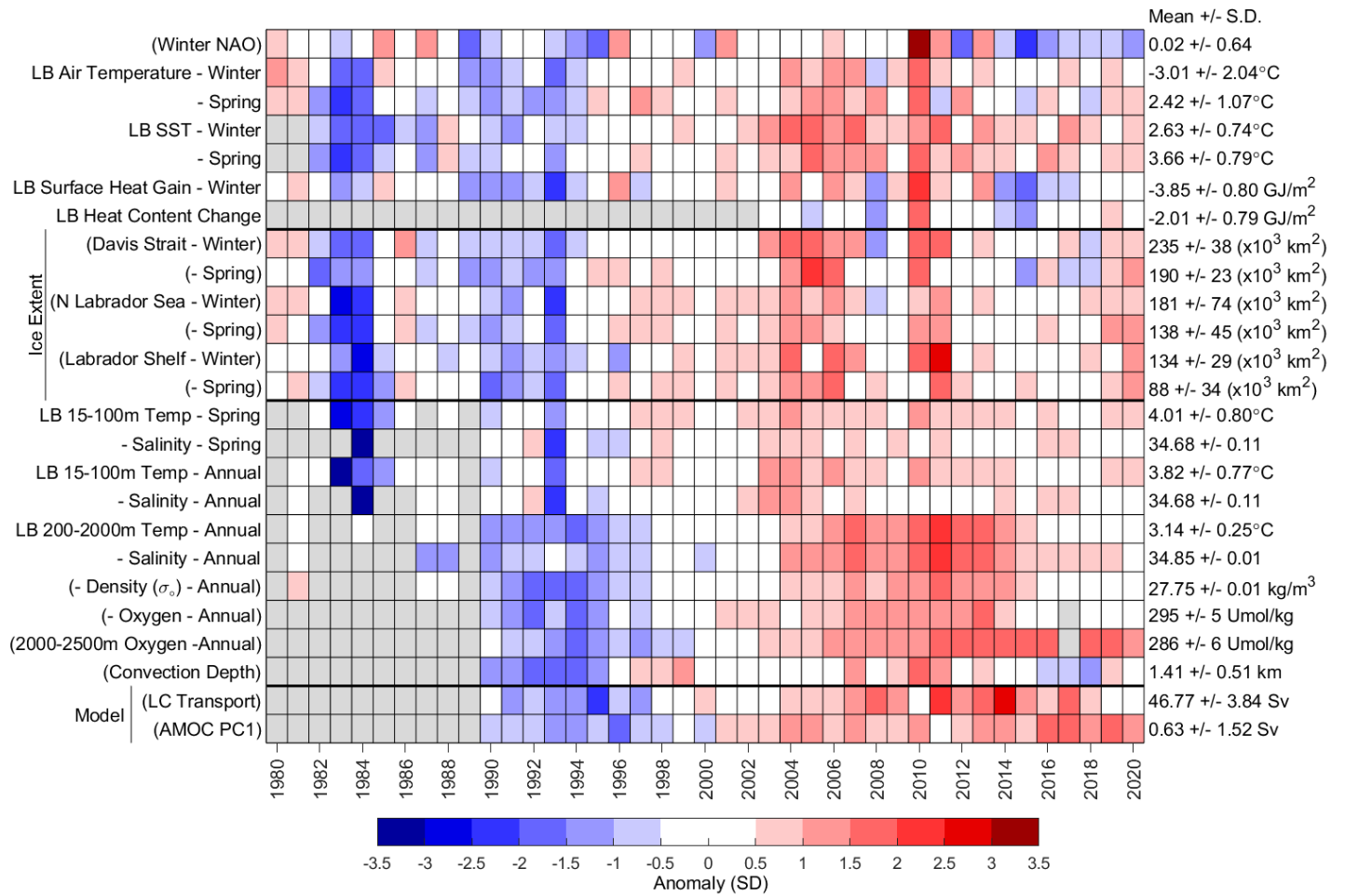
Figure 21. Scorecard for 1980-2020 oceanographic series. A grey cell indicates missing data, a white cell is a value within 0.5 SD of the long-term mean based on data from 1981–2010 when possible; a red cell indicates above normal conditions, and a blue cell below normal. Variables whose names appear in parentheses have reversed colour coding, whereby reds are lower than normal values that correspond to warm conditions. More intense colours indicate larger anomalies. Long-term means and standard deviations are shown on the right-hand side of the figure. North Atlantic Oscillation [NAO], Labrador Basin [LB], Labrador Current [LC].
