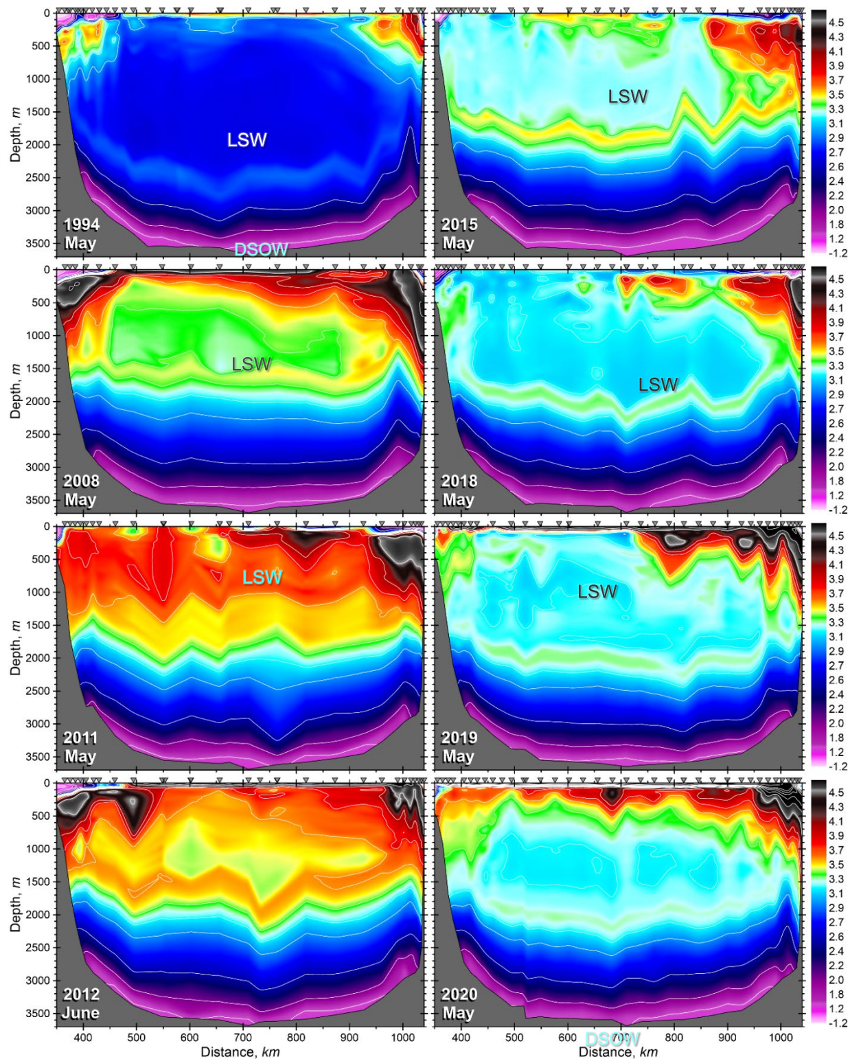
Figure 12. Distributions of potential temperature ( ^{\circ}\text{C} ) on the AR7W line across the Labrador Sea from annual spring-summer surveys in 1994, 2008, 2011, 2012, 2015, 2018, 2019 and 2020. Inverted triangles along the top of each panel indicate station locations. LSW, NEADW and DSOW indicate Labrador Sea Water, Northeast Atlantic Deep Water and Denmark Strait Overflow Water, respectively.
