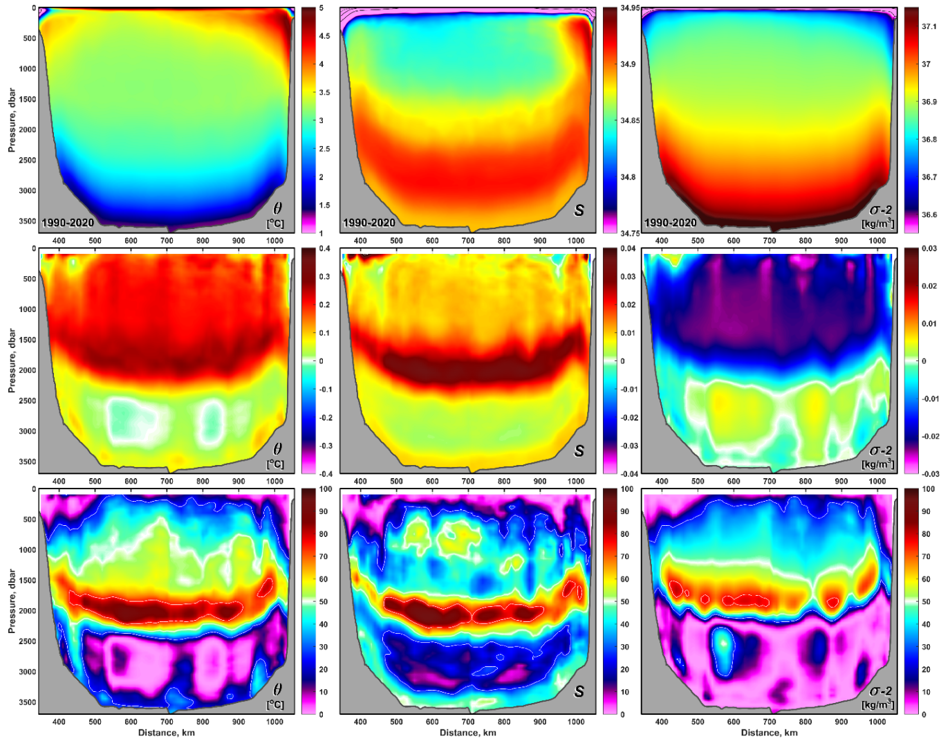
Figure 15. Climatological normals of temperature (upper left), salinity (upper central) and density (upper right) on the AR7W line for the period of 1990-2020, based on the entire collection of both Canadian and international Labrador Sea oceanographic survey data; the 1990-2020 period average rate of change (middle row, property changes rated to ten years) of temperature (left), salinity (central) and density (right), obtained by fitting linear trends the respective 31-year long time series constructed for each depth/pressure – distance bin within the active AR7W section plane; and the contributions (percentage) of the linear trend to the total variance for temperature (lower left), salinity (lower central) and density (lower right).
