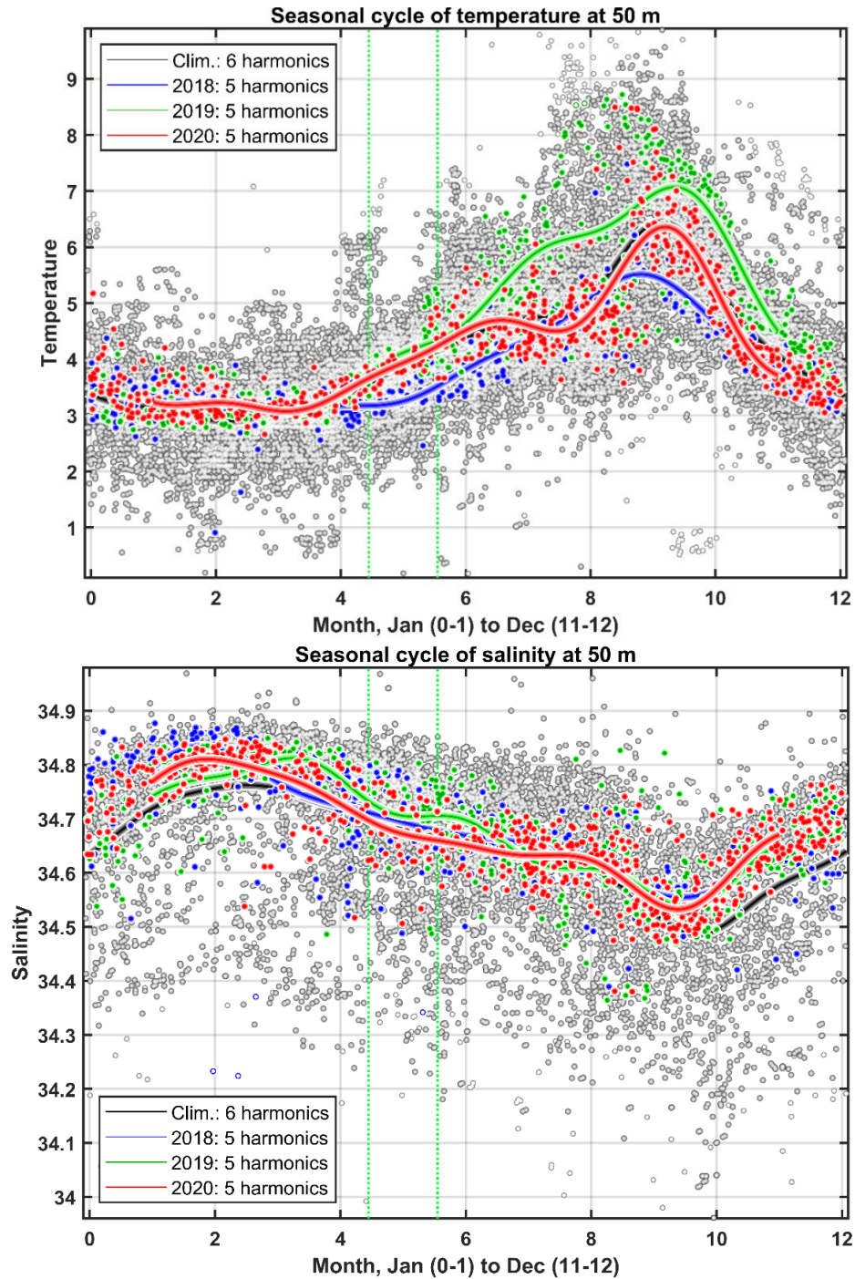
Figure 1. (c) Temperature (upper panel) and salinity (lower panel) measurements at 50 m in the central Labrador Sea for the period of 1948-2021 (note phase shift). The 2018, 2019 and 2020 data values are shown in blue, green and red, respectively. The black line represents all-data climatological, regular or normal seasonal cycle; the blue, green and red lines represent the 2018, 2019 and 2020 seasonal cycles, respectively. The vertical green dotted lines confine the May 15 to June 15 period.
