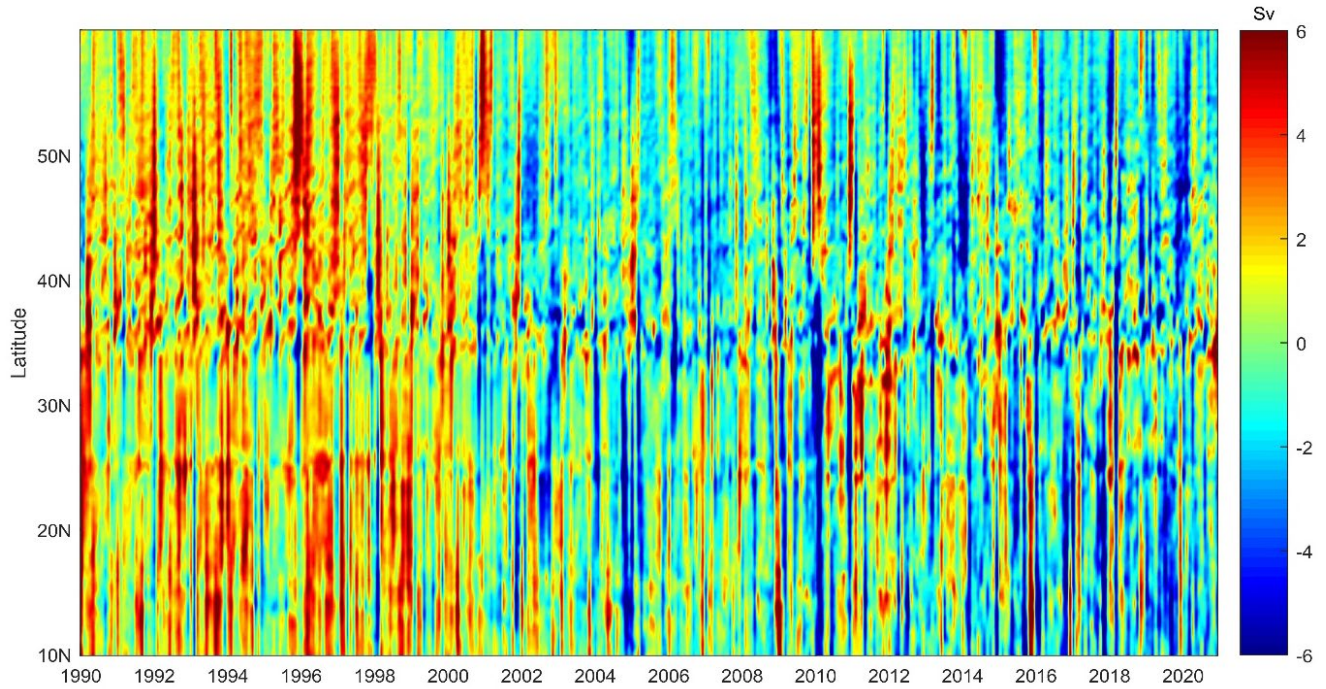
Figure 19. The AMOC anomalies at different latitudes with the seasonal cycles removed, but without detrending.
