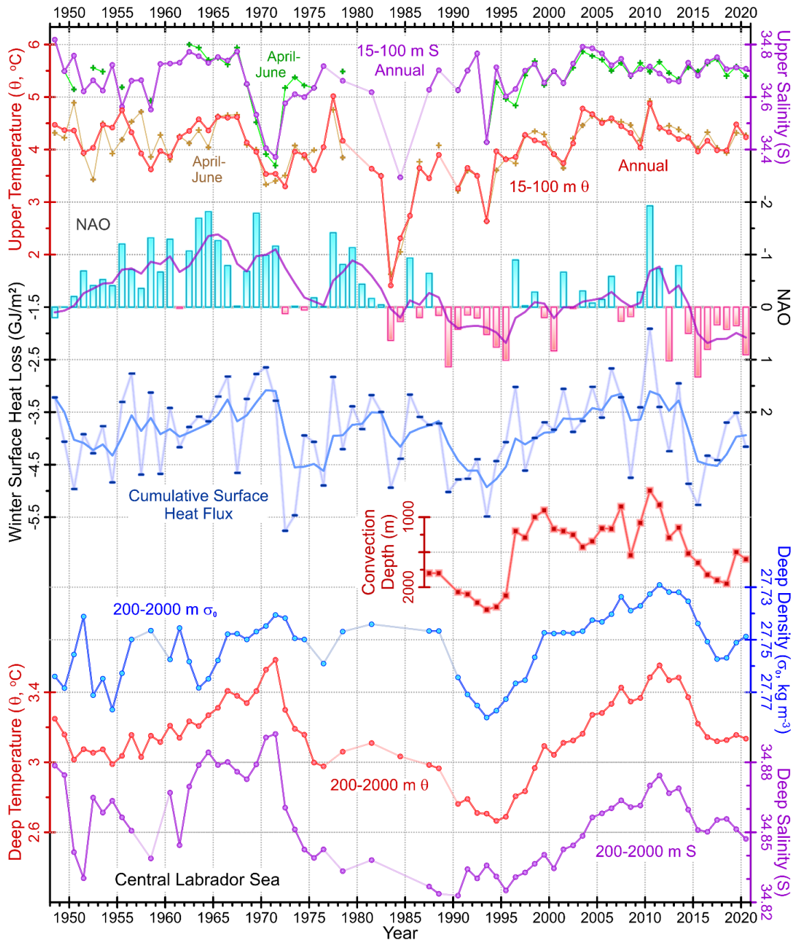
Figure 10. Key central Labrador Sea environmental state variables since 1948. From top down: annual and spring mean salinity (S) and temperature ( \theta ) averaged over the 15-100 m depth range; the normalized winter NAO index (bar graph, inverted scale); the NCEP reanalysis-based cumulative surface heat flux computed for the central Labrador Sea over individually-defined annual cooling seasons (blue); the two solid lines overlaying the NAO and heat flux graphs show five-back-point filtered series; annual mean seawater density ( \sigma_0 , referenced to 0 dbar), \theta and S averaged over the 200-2000 m depth range in the central Labrador Sea.
