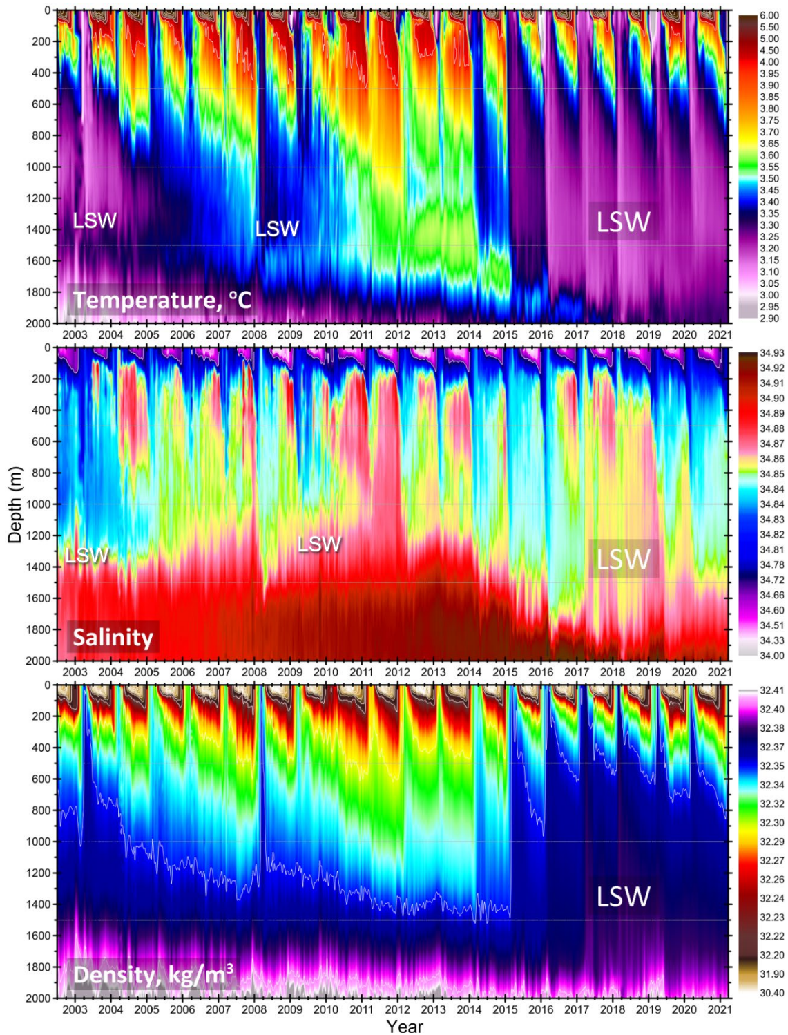
Figure 11. Temperature (upper), salinity (middle) and density (ref. to 1000 dbar; lower) in the central Labrador Sea created by averaging of the cleaned and corrected Argo float and shipboard data in 10-day time bins spaced at 5-day intervals (time range: 2002-2021, depth range: 0-2000 m, respectively).
