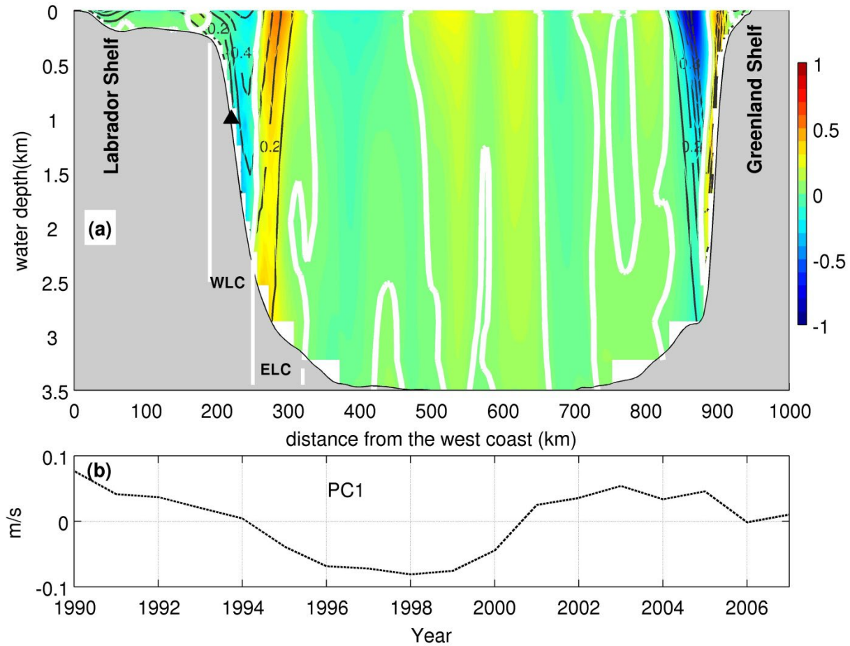
Figure 17. (a) EOF1 pattern of the normal velocities along AR7W (based on results from 1990 to 2007). The shaded areas represent the EOF pattern, bold white lines are zeros contours of the EOF pattern, the black labeled lines are the mean normal velocities (in m/s). Note: positive direction is northward. The black triangle indicates the location of the mooring referred to in the text.
