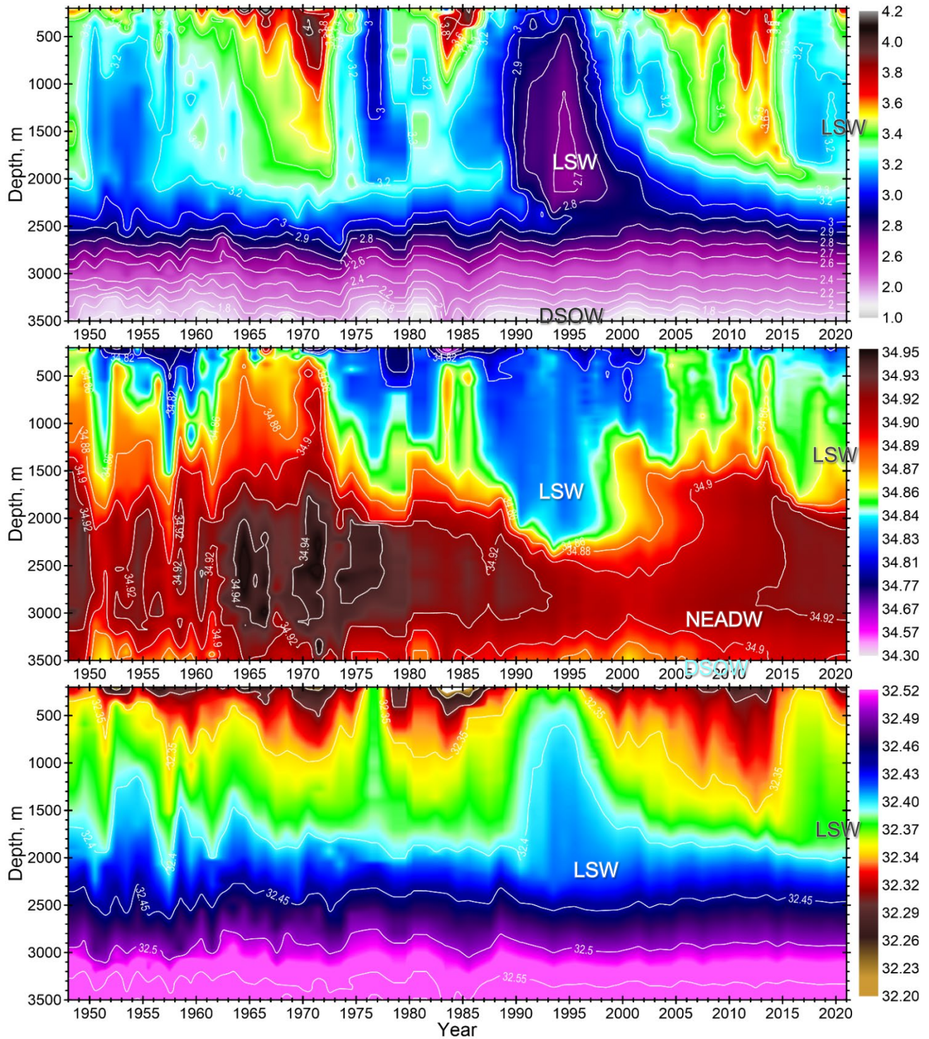
Figure 8. Annual temperature (upper panel), salinity (middle panel) and density (referenced to 1000 dbar pressure, lower panel) profiles in the central region of the Labrador Sea (time period: 1948-2020, depth range: 200-3500 m). The quality controlled observations were averaged annually for 1948-1987, in two steps: first, locally isobarically, and then, regionally isopycnally. For 1987-2020, the shipboard data were averaged mainly isopycnally, while Argo in the two-step process. LSW, NEADW and DSOW indicate Labrador Sea Water, Northeast Atlantic Deep Water and Denmark Strait Overflow Water, respectively.
