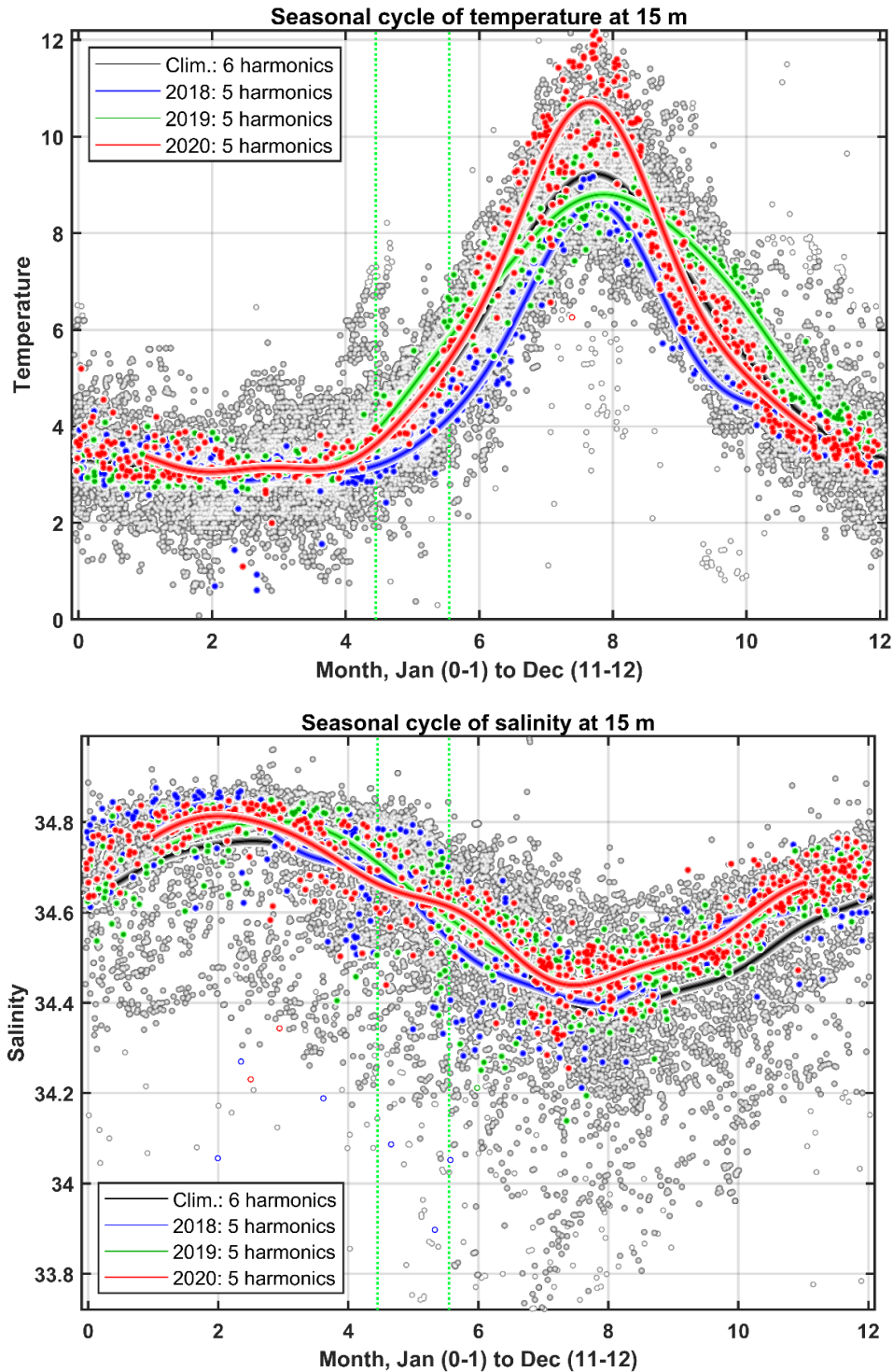
Figure 1. (b) Temperature (upper panel) and salinity (lower panel) measurements at 15 m in the central Labrador Sea for the period of 1948-2021. The 2018, 2019 and 2020 data values are shown in blue, green and red, respectively. The black line represents all-data climatological, regular or normal seasonal cycle; the blue, green and red lines represent the 2018, 2019 and 2020 seasonal cycles, respectively. The vertical green dotted lines confine the time period from May 15 to June 15.
