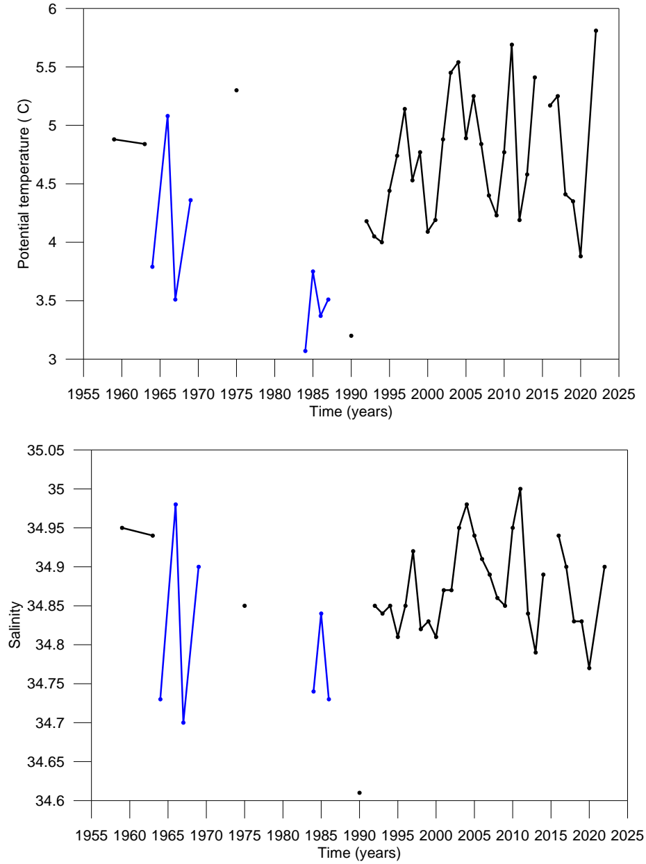
Figure 4. Mean potential temperature (°C, top) and salinity (bottom) for the depth range 75-200 m at Cape Desolation 3 (60.47°N, 50°W) June/July 1959-2022. Blue lines indicate observations obtained early in April.
