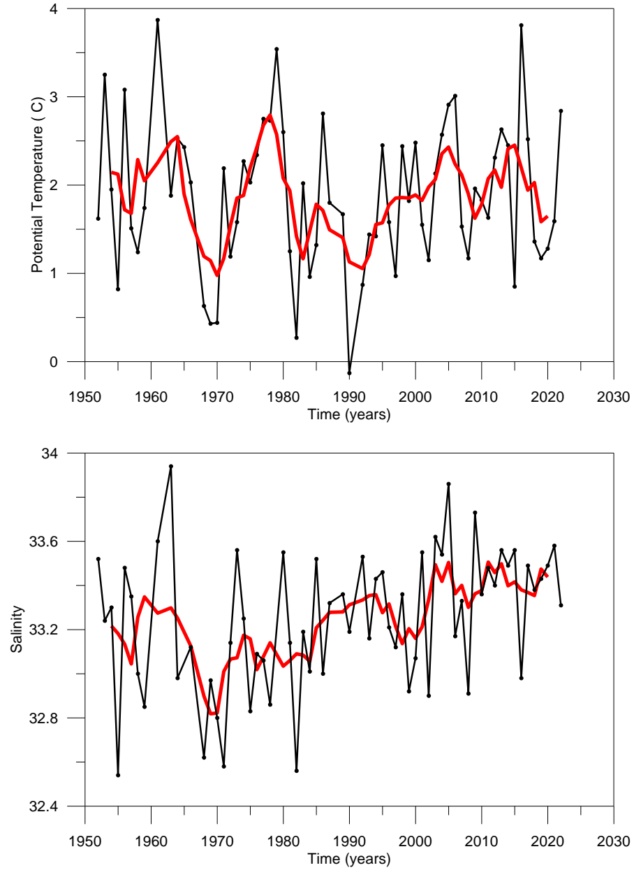
Figure 2. Time series of mean potential temperature (°C, top) and salinity (bottom) from the Fyllas Banke continental slope (station 4, 0-50 m) with measurements in June/July for the period 1952-2022. The red curve shows the 5 year running mean.
