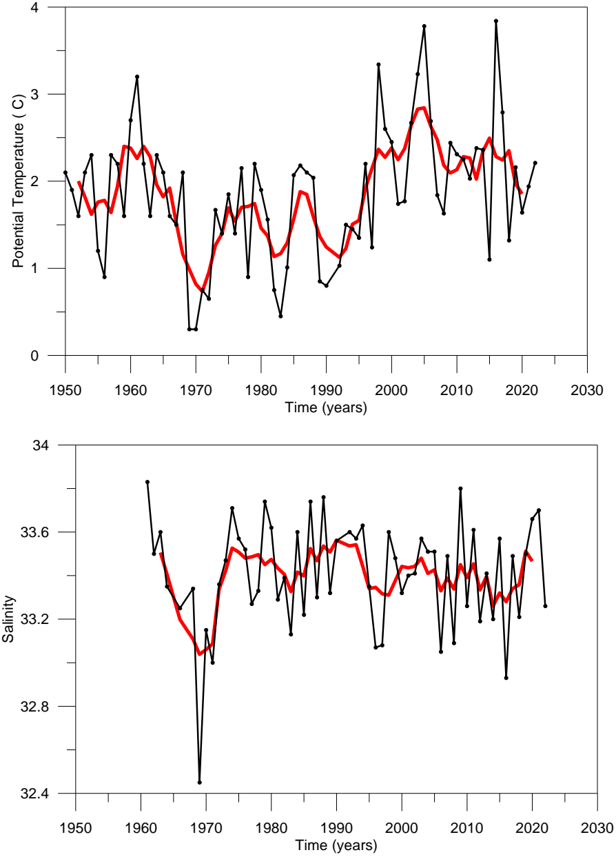
Figure 3. Time series of mean potential temperature (°C, top) and salinity (bottom) from the Fyllas Banke continental shelf (station 2, 0-40 m) with measurements in June/July for the period 1950-2022. The red curve shows the 5 year running mean.
