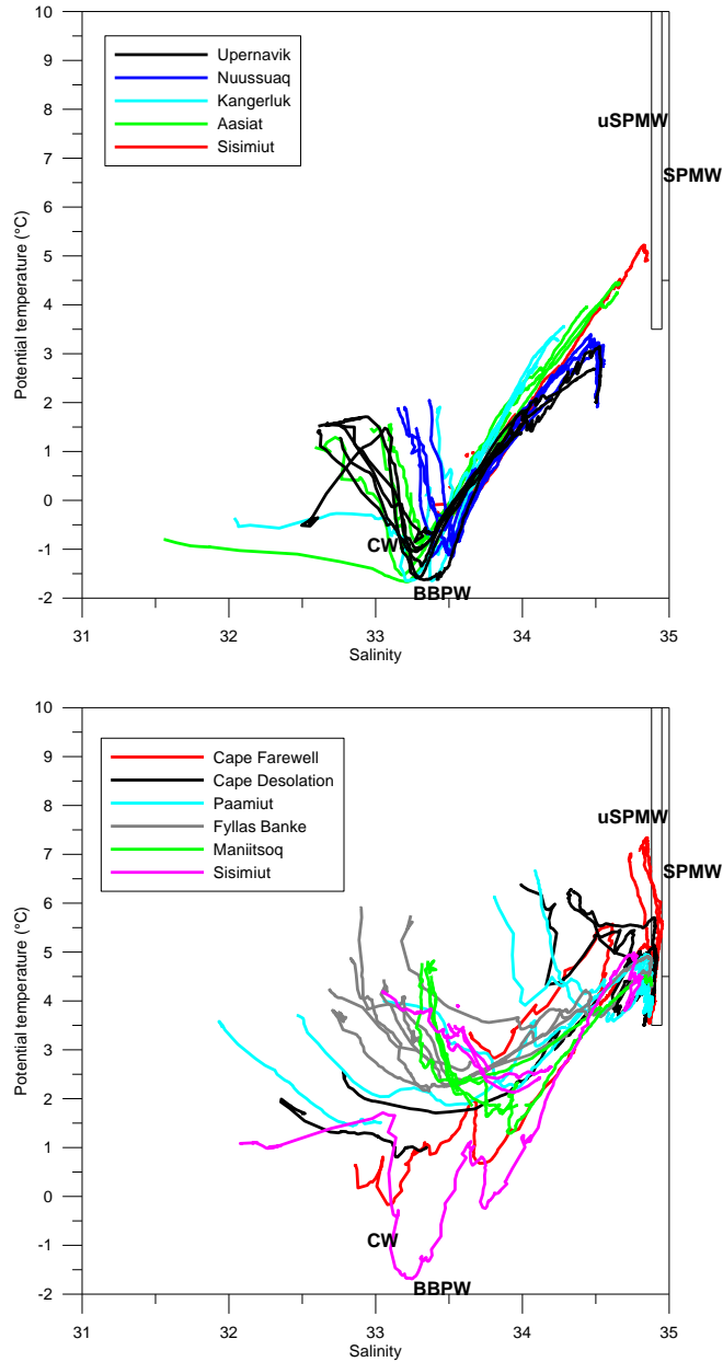
Figure 5. Potential temperature – salinity diagram showing every station occupied along the West Greenland continental shelf and slope during the June-July GINR surveys in 2022. Stations are color coded with respect to sections (see Figure legends and Figure 1). Also indicated are water masses that meet in the region: Coastal Water (CW), Subpolar Mode Water (SPMW), upper Subpolar Mode Water (upper SPMW), and Baffin Bay Polar Water (BBPW).
