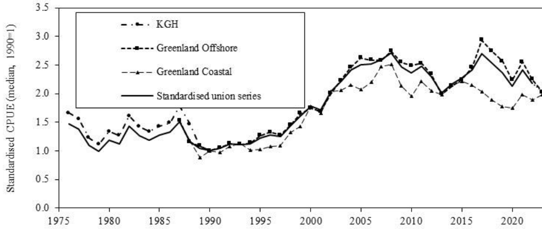
Figure 9. P. borealis in W. Greenland: standardized (1990=1) CPUE series from three fleets and a standardized union series 1976–2023. 2023 is on part-year’s data.
