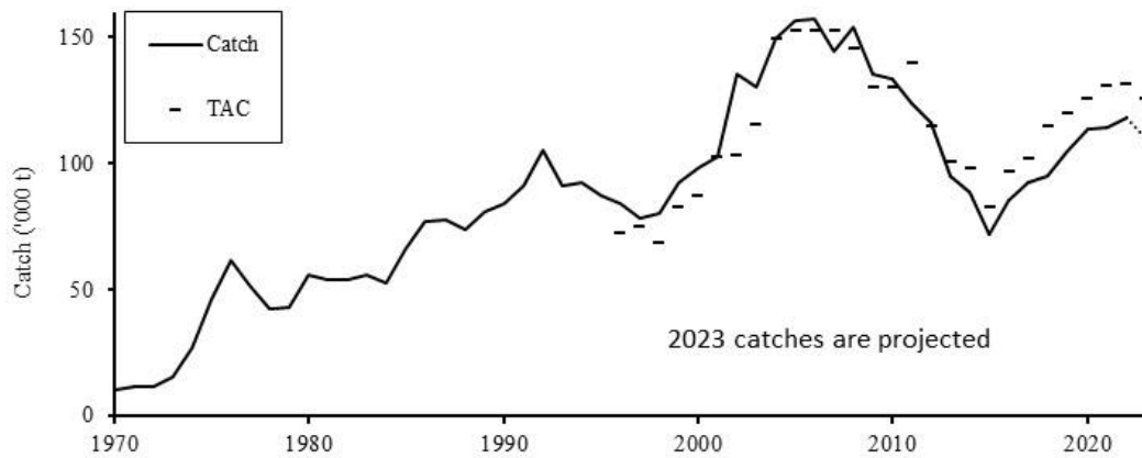
Figure 2. P. borealis in W. Greenland: Catches in NAFO Subarea 1 and Canadian SFA 1, 1970–2023. 2023 is projected catch.
