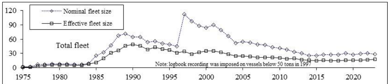
Figure 1a. P. borealis in W. Greenland: Nominal and effective sizes of the Greenland trawler fleet, 1975–2023, from logbook records.
