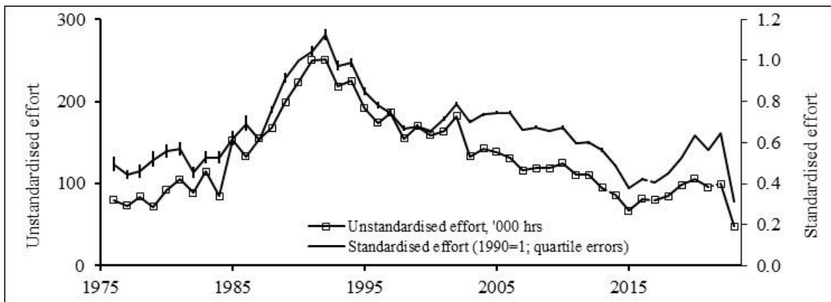
Figure 3. P. borealis in W. Greenland: Fishing effort applied in NAFO Subarea 1, 1970–2023. 2023 is on part-year's data.
