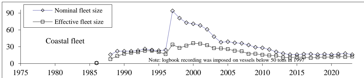
Figure 1c. P. borealis in W. Greenland: Nominal and effective sizes of the Greenland coastal trawler fleet, 1986–2023, from logbook records.
