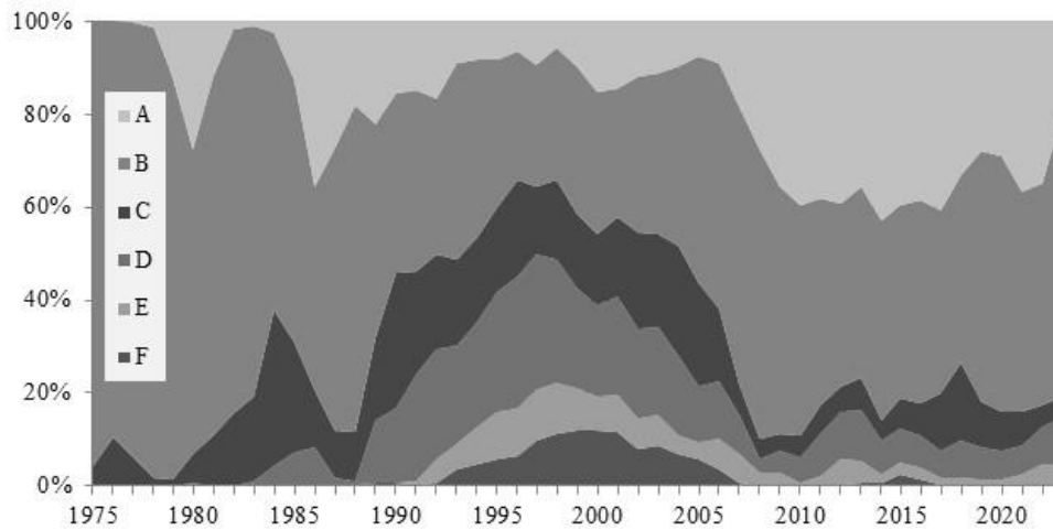
Figure 5b. P. borealis in W. Greenland: Distribution of the logbook-recorded catch between NAFO Divisions in Subarea 1 up to 76° N, 1975-2023.
