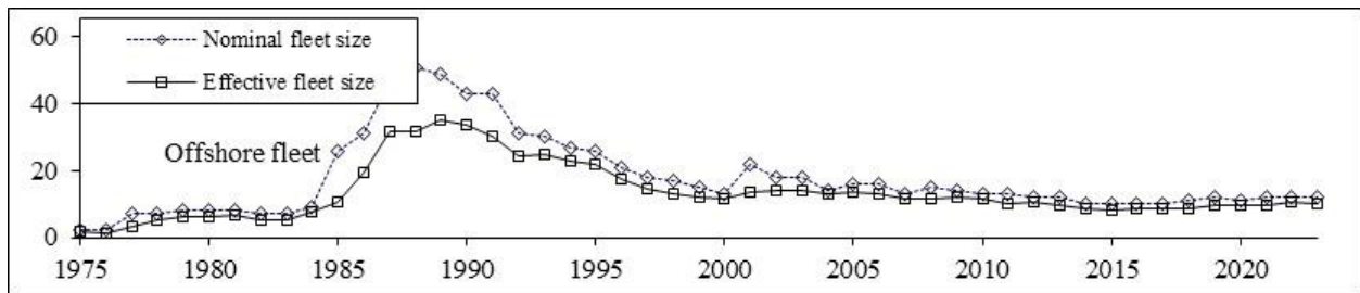
Figure 1b. P. borealis in W. Greenland: Nominal and effective sizes of the Greenland offshore trawler fleet, 1975–2023, from logbook records.
