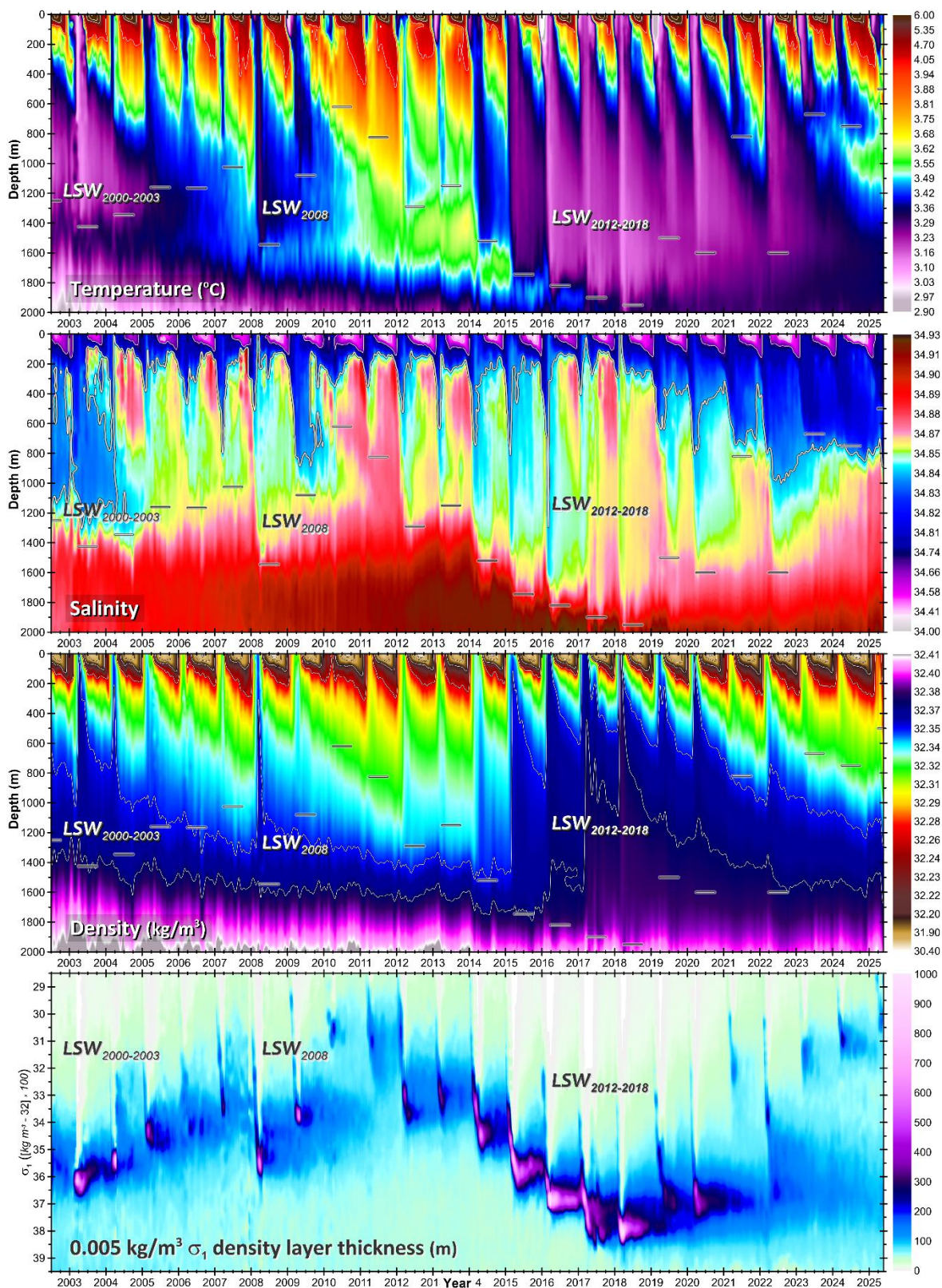
Figure 6. Central Labrador Sea temperature, salinity, density, and 0.005 \text{ kg/m}^3 density layer thickness based on quality-controlled and calibrated Argo float and ship-based observations. Short horizontal lines indicate the convection depths. Dots at 500, 1000 and 1500 m and 32.30 and 32.35 \text{kg/m}^3 indicate the dates of the time bins.
