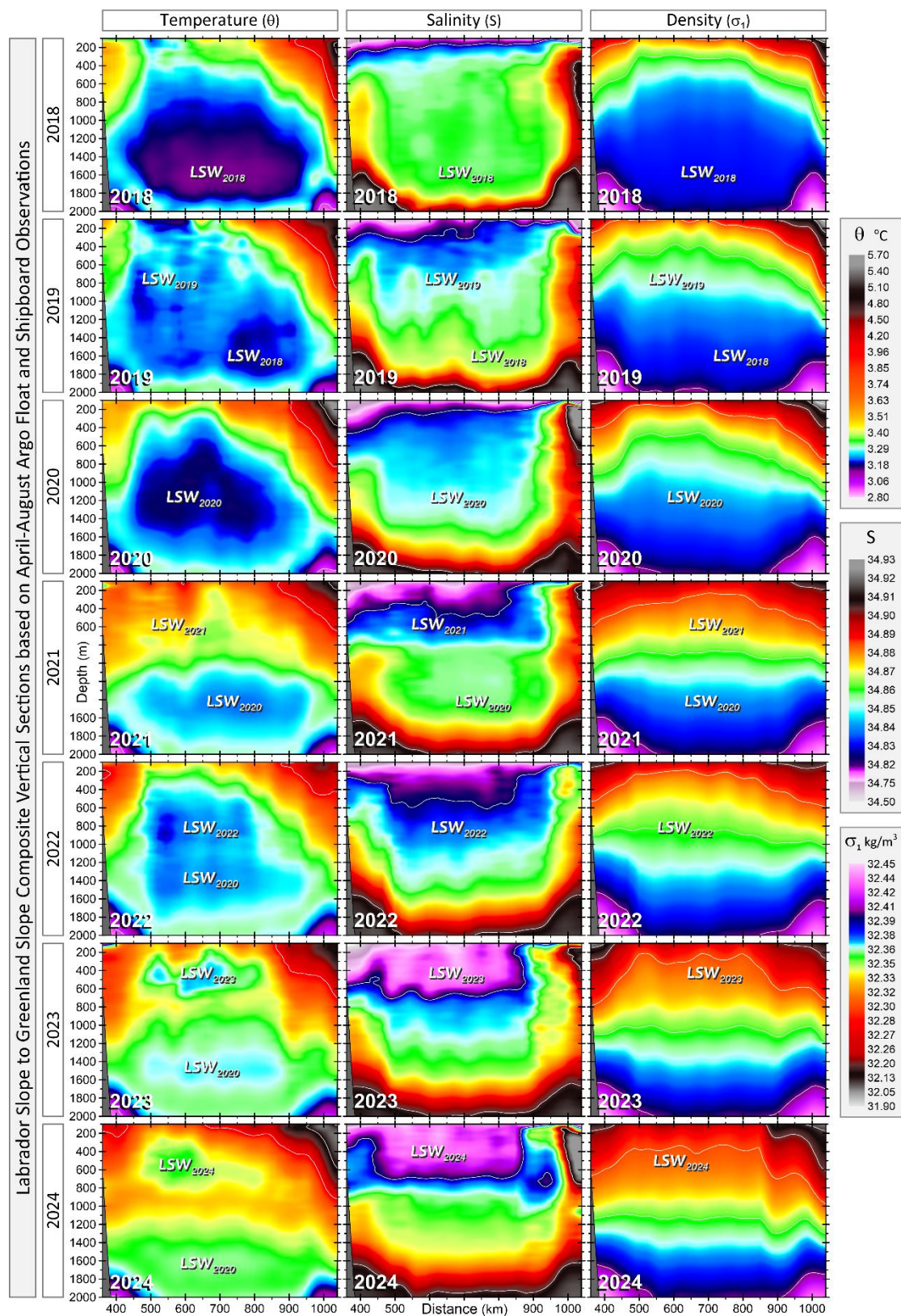
Figure 8. 2018-2024 post-convective (Apr-Aug) composite temperature, salinity, and density sections based, mostly , on the Argo float data, and, to a lesser degree , on the ship-based observations.
