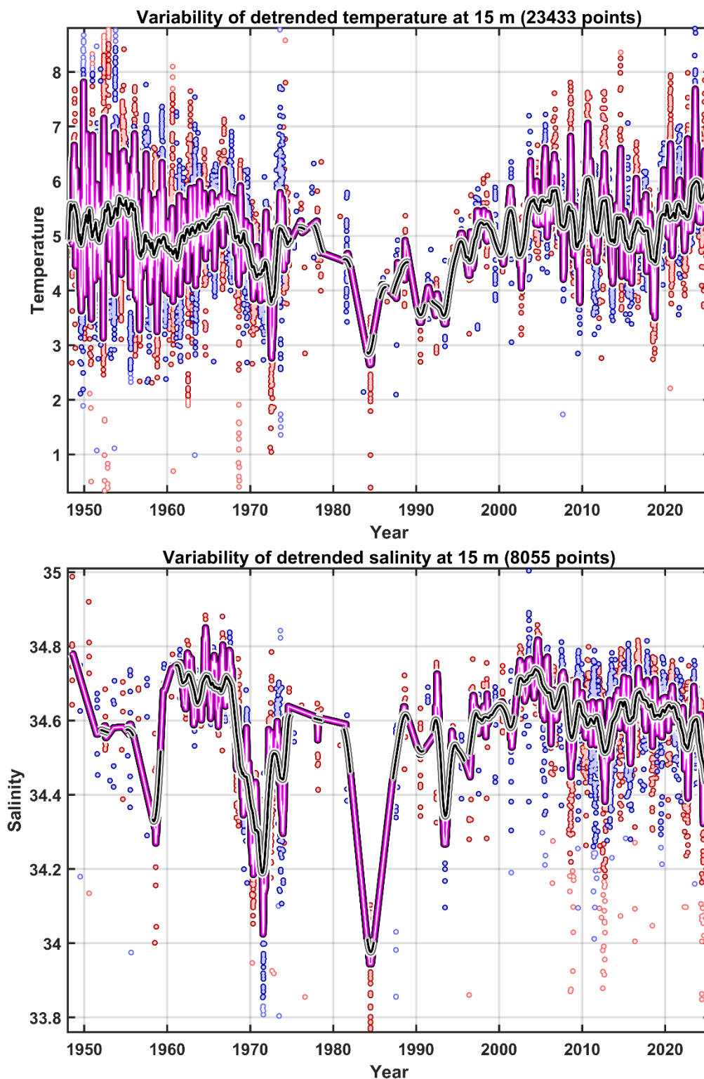
Figure 13. Temperature ( upper panel ) and salinity ( lower panel ) measurements at 15 m depth level in the central Labrador Sea for the period of 1948-2023 (Figure 1) with the seasonal cycle being removed from all individual observations. The data values for the even-numbered years (i.e., 1948, 1950, ..., 2020 and 2022) are shown with red dot clouds , for the odd-numbered years (i.e., 1949, 1951, ..., 2021 and 2023) with blue dot clouds . The purple-padded and black lines represents one-month and one-year low-pass filtered data, respectively.
