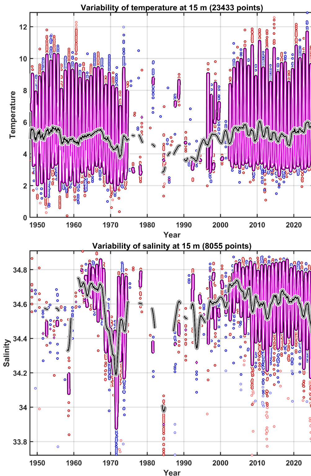
Figure 12. Temperature ( upper panel ) and salinity ( lower panel ) measurements at 15 m depth level in the central Labrador Sea for the period of 1948-2023 (Figure 1) with respect to decimal year. The data values for the even-numbered years (i.e., 1948, 1950, ..., 2020 and 2022) are shown with red dot clouds , for the odd-numbered years (i.e., 1949, 1951, ..., 2021 and 2023) with blue dot clouds . The purple-padded and black lines represents one-month and one-year low-pass filtered data, respectively.
