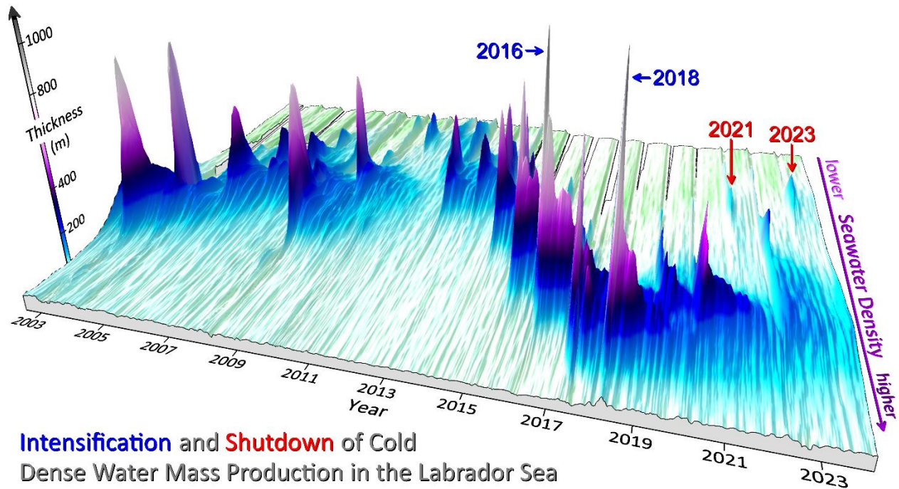
Figure 7. 0.005 kg/m 3 density layer thickness based on quality-controlled and calibrated Argo float and ship-based observations. The values presented in this figure are analogous to those shown in the lower panel of Figure 6. Here, the changes of density layer thickness across the density and time bins allow us to closely follow how the most voluminous LSW class since the 1990s developed over the 2012-2018 period, and sized to be renewed and replenished afterwards.
