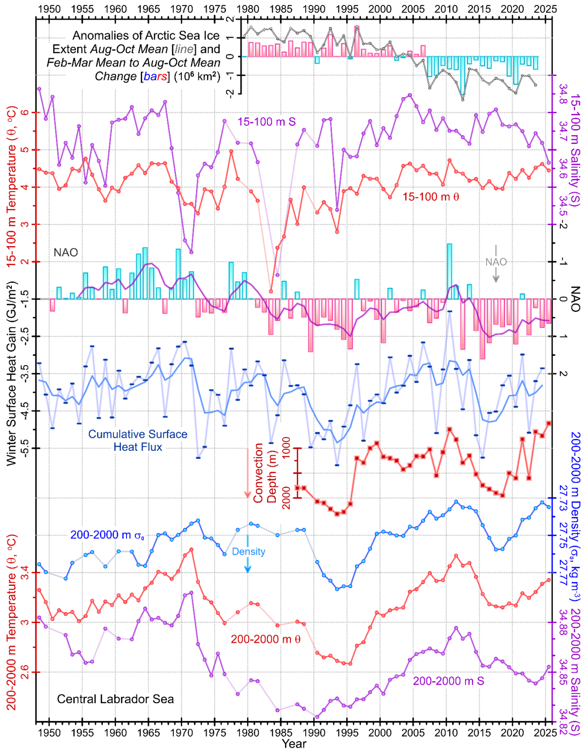
Figure 10. Top-down: The Aug-Oct Arctic sea ice extent, and Feb-Mar to Aug-Oct extent change anomalies; the 1948-2025 central Labrador Sea (CLS) 15-100 m vertically and annually averaged de-seasoned salinity (S) and temperature ( \theta ); the winter NAO index (inverted); the CLS surface heat flux integrated over individually defined cooling seasons (blue); the low-pass left-side-window filtered NAO and surface heat flux (solid lines); the convection depth; the CLS 200-2000 m vertically and annually averaged density ( \sigma_{\theta} , referenced to 0 dbar), \theta and S.
