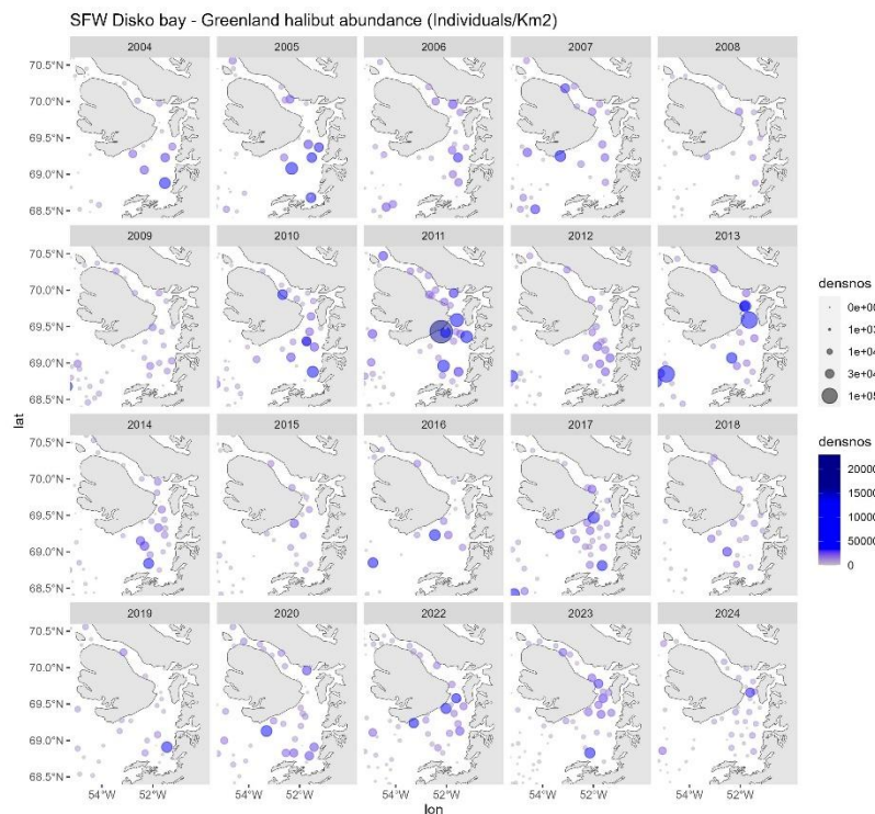
Figure 4. Abundance distribution (individuals/km 2 ) from the Disko Bay part of the GINR Shrimp and fish survey.
