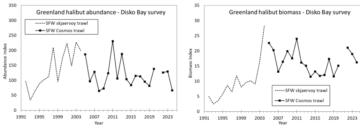
Figure 2. Trawl survey (SFW) in the Disko Bay: Abundance (left) and biomass (right).
