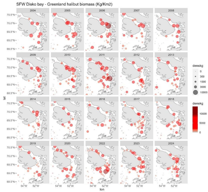
Figure 5. Biomass distribution (Kg/km 2 ) from the Disko Bay part of the GINR Shrimp and fish survey.
