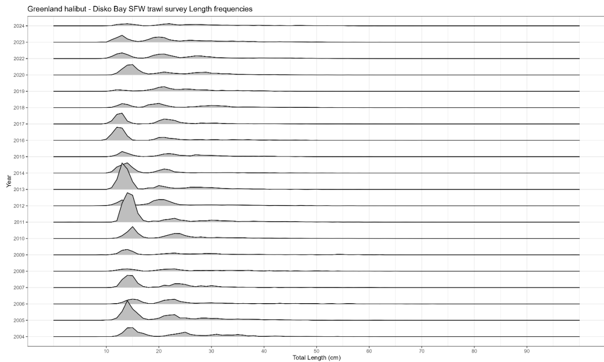
Figure 3. Greenland halibut length frequency distributions from the Disko Bay part of the GINR Shrimp and fish survey.
