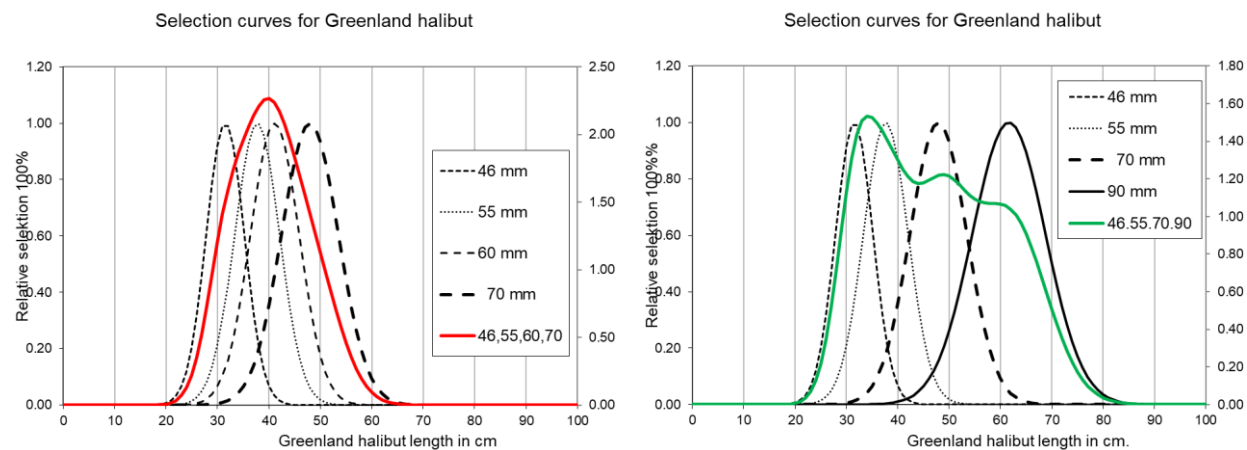
Figure 11. Relative selection curves (gillnet) for Greenland halibut. The combined selection curve for the original gillnet design (46,55,60,70) is shown in red (left figure) and in a more optimal combination in green (right).
