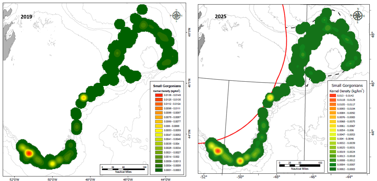
Figure 62. Kernel density biomass surfaces of the Small Gorgonian Coral Functional Group in the NAFO Regulatory Area comparing the surface created in 2019 with that created in 2025.
