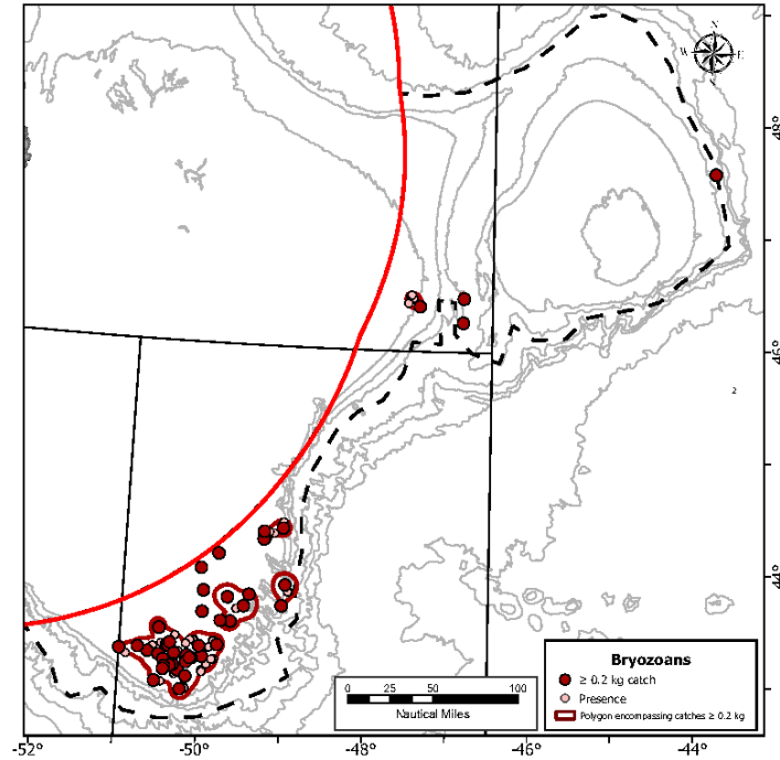
Figure 80. Illustration of the Erect Bryozoan Functional Group VME polygons (red outline), catches \geq 0.20 kg (solid red circles) and catches within the VME polygons but at lower catch weights (solid pink circles). Black dashed line represents the NAFO fishing footprint; solid red line represents the Canadian Exclusive Economic Zone.
