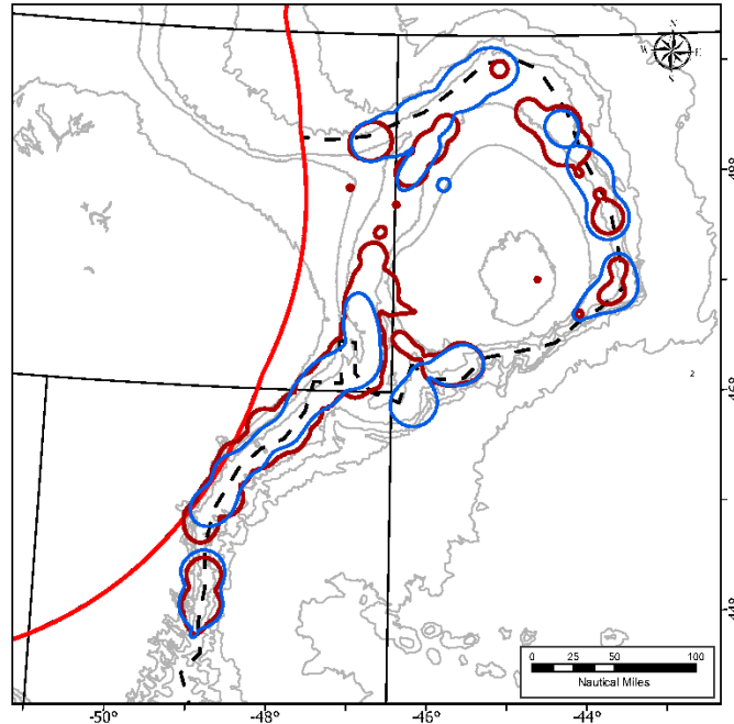
Figure 24. Comparison of the Astrophorina sponge VME polygons (red outline) with the Large-Size Sponge VME polygons analyzed above (blue outline). Black dashed line represents the NAFO fishing footprint; solid red line represents the Canadian Exclusive Economic Zone.
