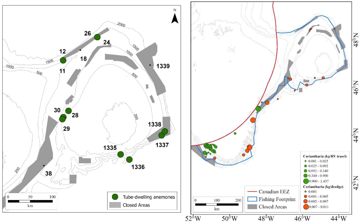
Figure 87. Left panel. Presence of Tube-Dwelling ( Ceriantharia ) Anemones on video and photographic transects collected from the Flemish Cap area in 2009 and 2010. Right panel. Relative biomass of Ceriantharia collected during the NEREIDA surveys between 2009-2010 using a rock dredge (red) and EU-Spain research trawl surveys between 2006-2024 (green).
