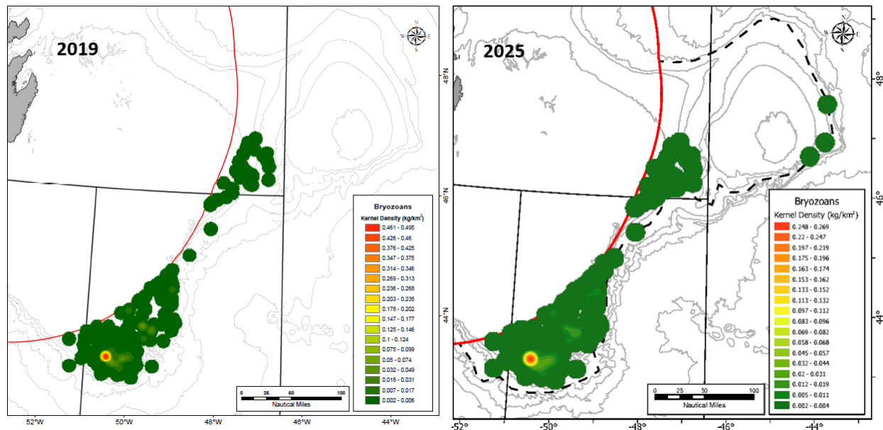
Figure 77. Kernel density biomass surface of the Erect Bryozoan Functional Group in the NAFO Regulatory Area comparing the surface created in 2019 with that created in 2025.
