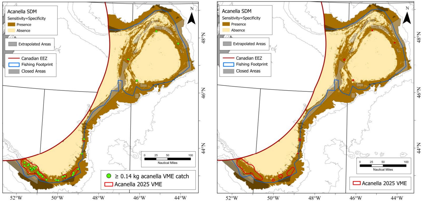
Figure 63. Left Panel. The 2025 Acanella arbuscula KDE VME polygons (Kenchington et al., 2025) superimposed on the SDM for Acanella arbuscula created with a threshold optimised to ensure that resulting Sensitivity=Specificity (Murillo et al., 2025). The location of research vessel survey catches greater than or equal to 0.14 kg are indicated. Right Panel. The 2025 Acanella arbuscula KDE VME polygons (Kenchington et al., 2025) superimposed on the SDM for Acanella arbuscula created with a threshold optimised to ensure that resulting Sensitivity=Specificity (Murillo et al., 2025).
