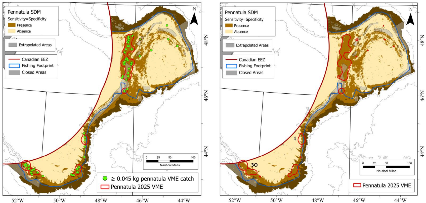
Figure 46. Left Panel. The 2025 Pennatula KDE VME polygons (Kenchington et al., 2025) superimposed on the SDM for Pennatula created with a threshold optimised to ensure that resulting Sensitivity=Specificity (Murillo et al., 2024). The location of research vessel survey catches greater than or equal to 0.045 kg are indicated. Right Panel. The 2025 Pennatula KDE VME polygons (Kenchington et al., 2025) superimposed on the SDM for Pennatula created with a threshold optimised to ensure that resulting Sensitivity=Specificity (Murillo et al., 2024). Numbers indicate the Vulnerable Marine Ecosystem Area Closures referenced in Article 17.3 of the NAFO Conservation and Enforcement Measures (NAFO, 2025) and serve to identify the 2025 KDE VME polygons that warrant further examination for modifications.
