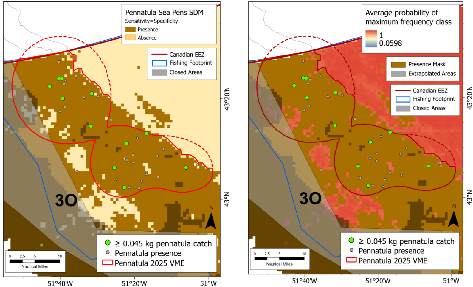
Figure 49. Area 30. Left Panel. Map of the proposed modification (solid red line) of the 2025 Pennatula KDE VME polygon (red dashed lines) and showing the underlying SDM (brown area showing predicted presence of Pennatula ). Right Panel. Map of the proposed modification (solid red line) of the 2025 Pennatula KDE VME polygon (red dashed lines) near Area 30 in relation to the average probability of the maximum frequency class for absence values from 10 SDM runs for Pennatula (Murillo et al., 2024). Closed areas are indicated in grey shading. Catches of \geq 0.045 kg, the threshold for the KDE analyses, and all other catches with < 0.045 kg are shown.
