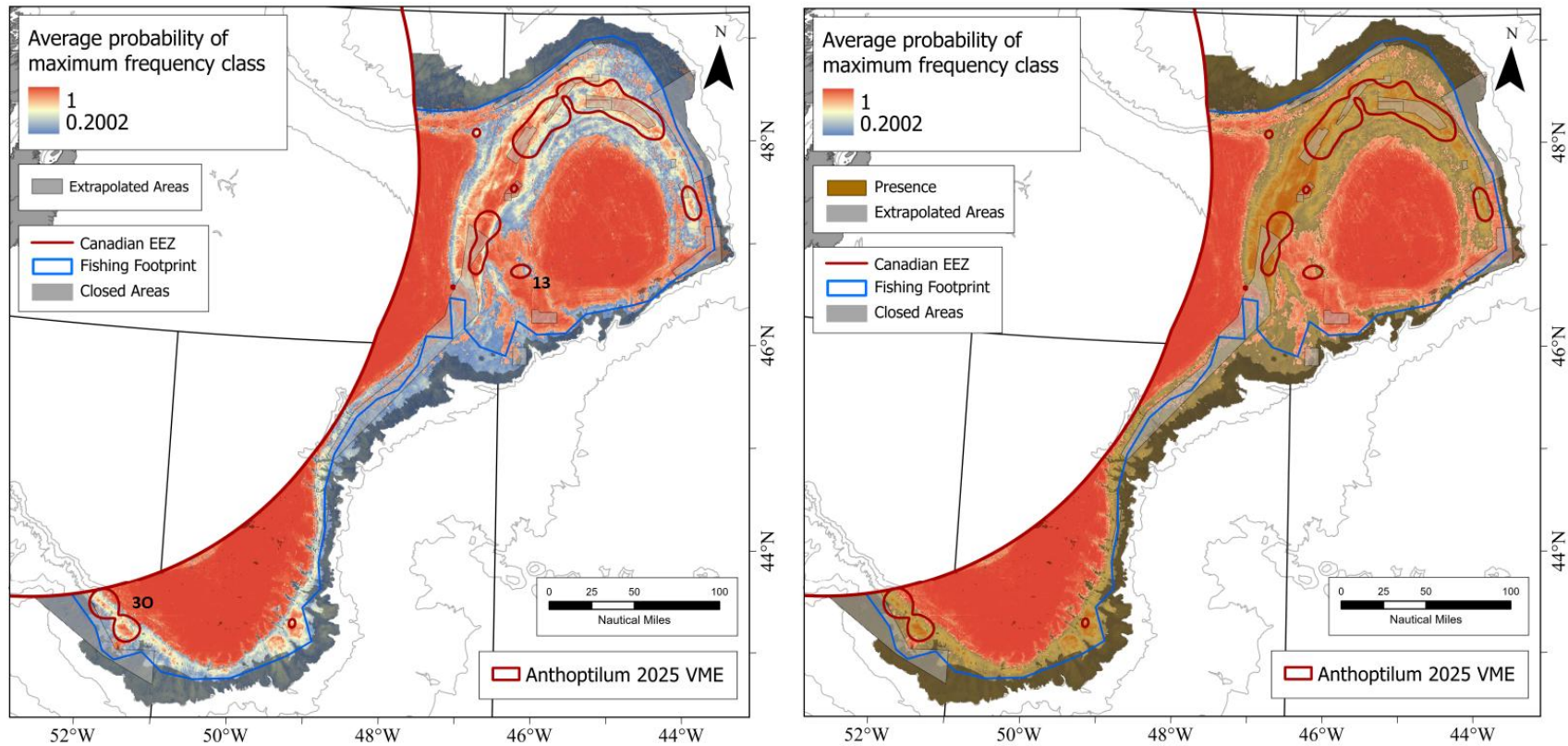
Figure 35. Left Panel. The 2025 Anthoptilum KDE VME polygons (Kenchington et al., 2025) superimposed on the average probability of the maximum frequency class (presence or absence) from 10 SDM runs for Anthoptilum (Murillo et al., 2024). Numbers indicate the Vulnerable Marine Ecosystem Area Closures referenced in Article 17.3 of the NAFO Conservation and Enforcement Measures (NAFO, 2025) and serve to identify the 2025 KDE VME polygons that warrant further examination for potential modifications. Right Panel. The 2025 Anthoptilum KDE VME polygons (Kenchington et al., 2025) superimposed on the average probability of the maximum frequency class (presence or absence) from 10 SDM runs for Anthoptilum which itself is superimposed with a 30% transparent overlay showing areas where the SDM predicts presence for the Anthoptilum created with a threshold optimised to ensure that resulting Sensitivity=Specificity (Murillo et al., 2024).
