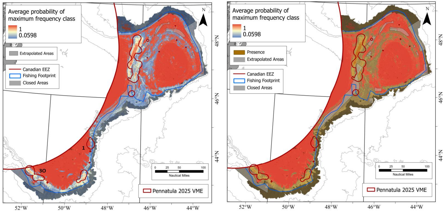
Figure 47. Left Panel. The 2025 Pennatula KDE VME polygons (Kenchington et al., 2025) superimposed on the average probability of the maximum frequency class (presence or absence) from 10 SDM runs for Pennatula (Murillo et al., 2024). Numbers indicate the Vulnerable Marine Ecosystem Area Closures referenced in Article 17.3 of the NAFO Conservation and Enforcement Measures (NAFO, 2025) and serve to identify the 2025 KDE VME polygons that warrant further examination for potential modifications. Right Panel. The 2025 Pennatula KDE VME polygons (Kenchington et al., 2025) superimposed on the average probability of the maximum frequency class (presence or absence) from 10 SDM runs for Pennatula which itself is superimposed with a 30% transparent overlay showing areas where the SDM predicts presence for Pennatula created with a threshold optimised to ensure that resulting Sensitivity=Specificity (Murillo et al., 2024).
