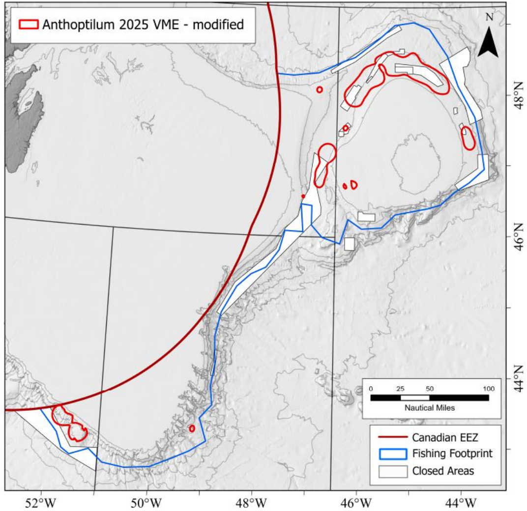
Figure 39. Map of the proposed Anthoptilum KDE VME polygons after consideration of modifications based on the SDM for Anthoptilum (Murillo et al., 2024). Closed areas are indicated in white (NAFO, 2025).
