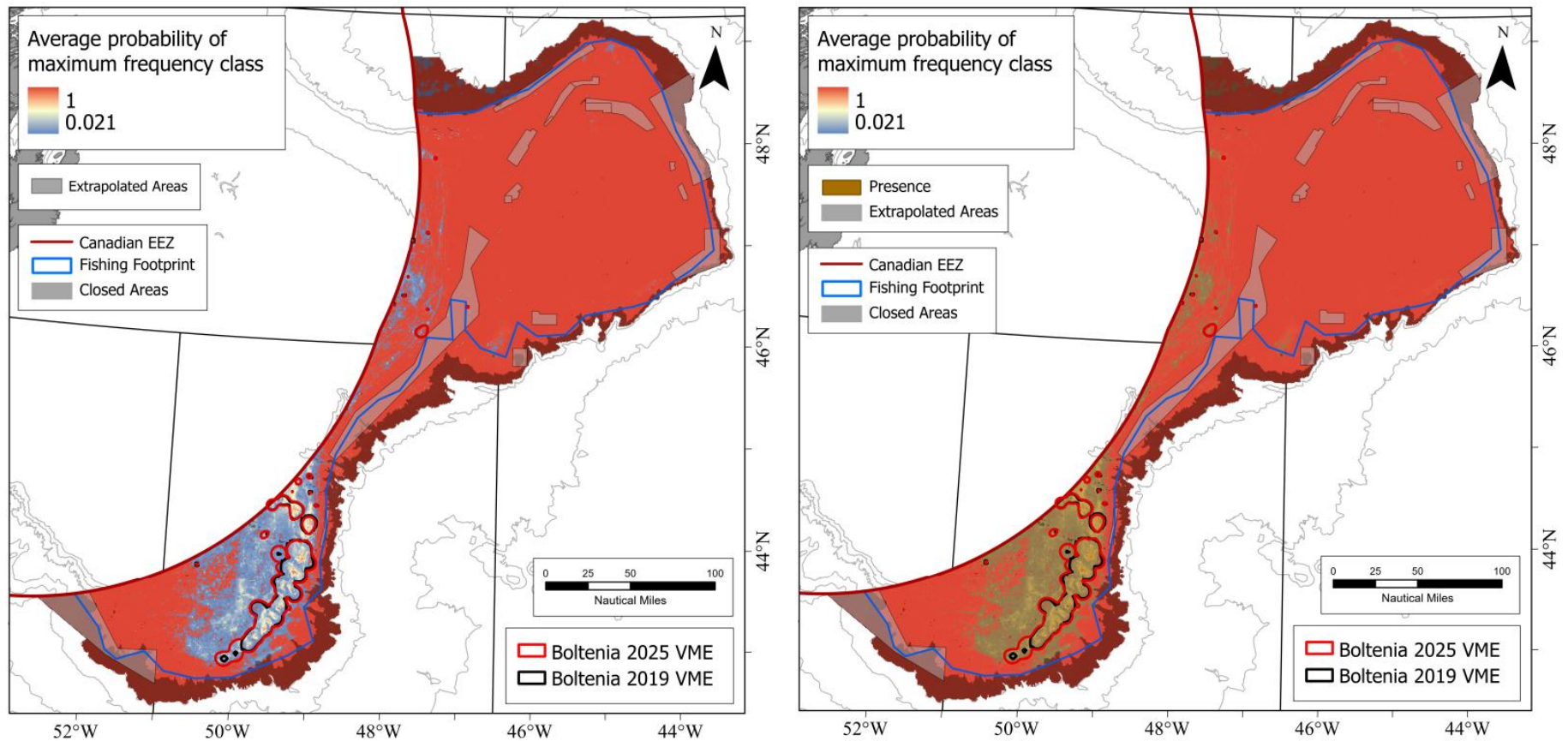
Figure 79. Left Panel. The 2025 (Kenchington et al., 2025) and 2019 clipped (Kenchington et al. 2019) Sea Squirrel ( Boltenia ) KDE VME polygons superimposed on the average probability of the maximum frequency class (presence or absence) from 10 SDM runs for the Sea Squirrel ( Boltenia ) (Murillo et al., 2025). Right Panel. The 2025 (Kenchington et al., 2025) and 2019 clipped (Kenchington et al. 2019) Sea Squirrel ( Boltenia ) KDE VME polygons superimposed on the average probability of the maximum frequency class (presence or absence) from 10 SDM runs for the Sea Squirrel ( Boltenia ) which itself is superimposed with a 30% transparent overlay showing areas where the SDM predicts presence for the Sea Squirrel ( Boltenia ) created with a threshold optimised to ensure that resulting Sensitivity=Specificity (Murillo et al., 2025).
