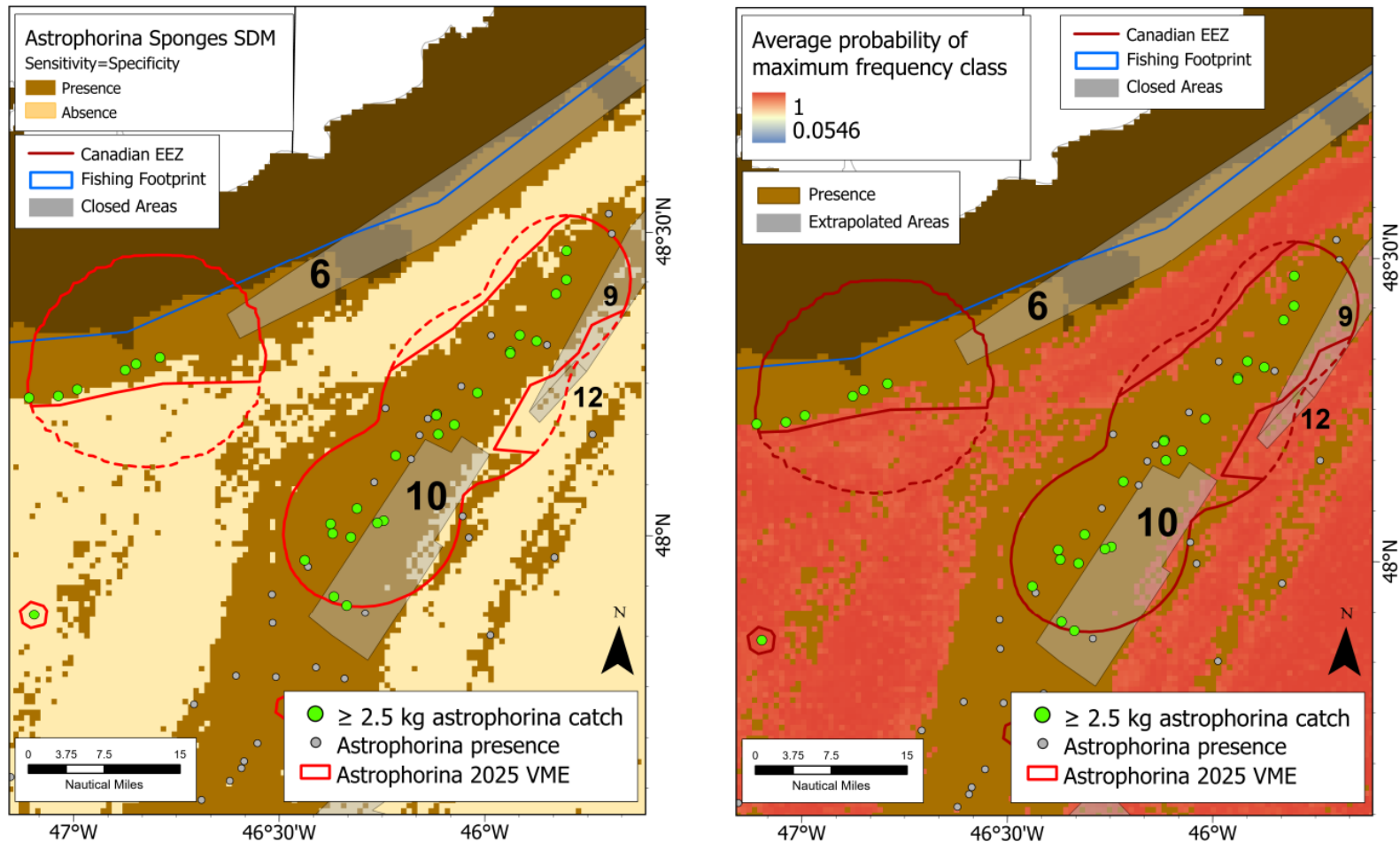
Figure 28. Areas 6 and 10. Left Panel. Map of the proposed modification (solid red line) of the 2025 Astrophorina Sponge KDE VME polygon (red dashed lines) and showing the underlying SDM (brown area showing predicted presence of Astrophorina Sponges). Right Panel. Map of the proposed modification (solid red line) of the 2025 Astrophorina Sponge KDE VME polygon (red dashed lines) near Areas 6 and 10 in relation to the average probability of the maximum frequency class for absence values from 10 SDM runs for the Astrophorina Sponges (Murillo et al., 2024). Closed areas are indicated in grey shading. Catches of \geq 2.5 kg, the threshold for the KDE analyses, and all other catches with < 2.5 kg are shown.
