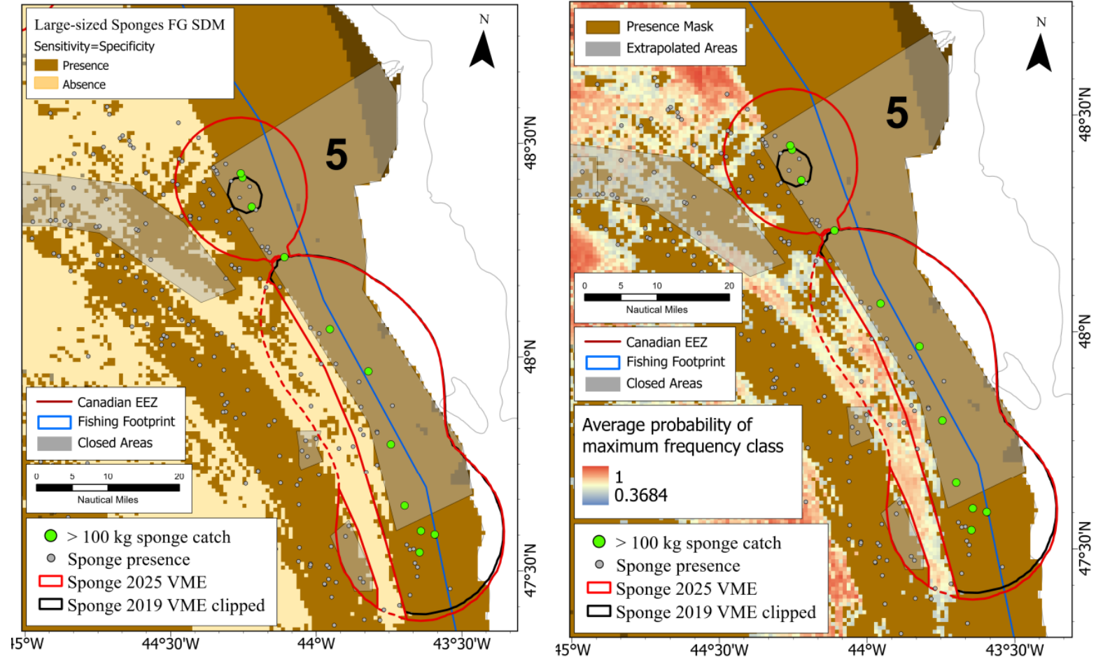
Figure 8. Area 5. Left Panel. Map of the proposed modification (solid red line) of the 2025 Large-Sized Sponge KDE VME polygon (red dashed lines) near Area 5 in relation to the 2019 accepted KDE VME polygon (solid black line) and showing the underlying SDM (brown area showing predicted presence of Large-Sized Sponges). Right Panel. Map of the proposed modification (solid red line) of the 2025 Large-Sized Sponge KDE VME polygon (red dashed lines) near Area 5 in relation to the 2019 accepted KDE VME polygon (solid black line) and showing the average probability of the maximum frequency class for absence values from 10 SDM runs for the Large-Size Sponge Functional Group (Murillo et al., 2024). Closed areas are indicated in grey shading. Catches of \geq 100 kg, the threshold for the KDE analyses, and all other catches with < 100 kg are shown).
