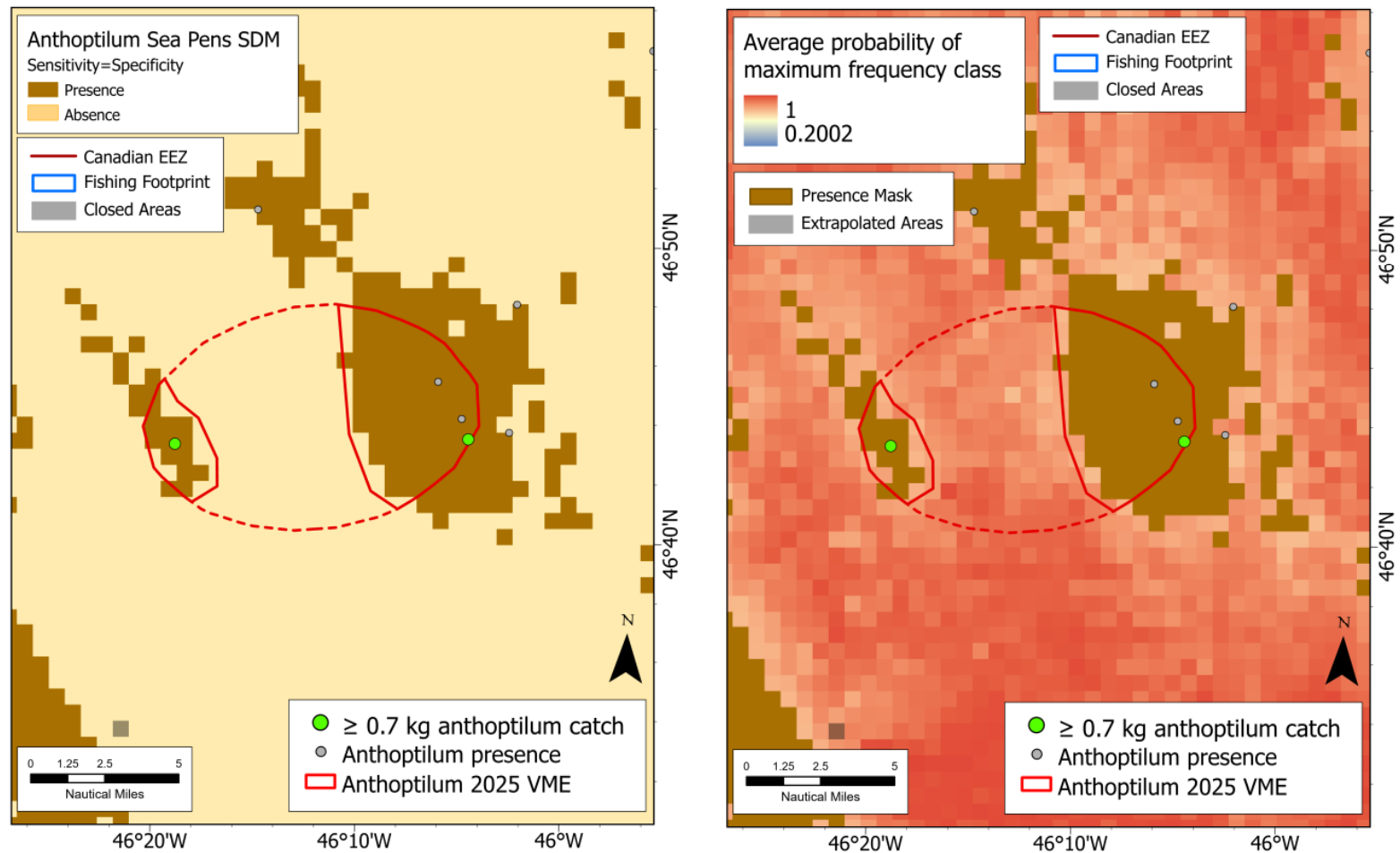
Figure 38. Area 13. Left Panel. Map of the proposed modification (solid red line) of the 2025 Anthoptilum KDE VME polygon (red dashed lines) and showing the underlying SDM (brown area showing predicted presence of Anthoptilum ). Right Panel. Map of the proposed modification (solid red line) of the 2025 Anthoptilum KDE VME polygon (red dashed lines) near Area 13 in relation to the average probability of the maximum frequency class for absence values from 10 SDM runs for Anthoptilum (Murillo et al., 2024). Closed areas are indicated in grey shading. Catches of \geq 0.7 kg, the threshold for the KDE analyses, and all other catches with < 0.7 kg are shown.
