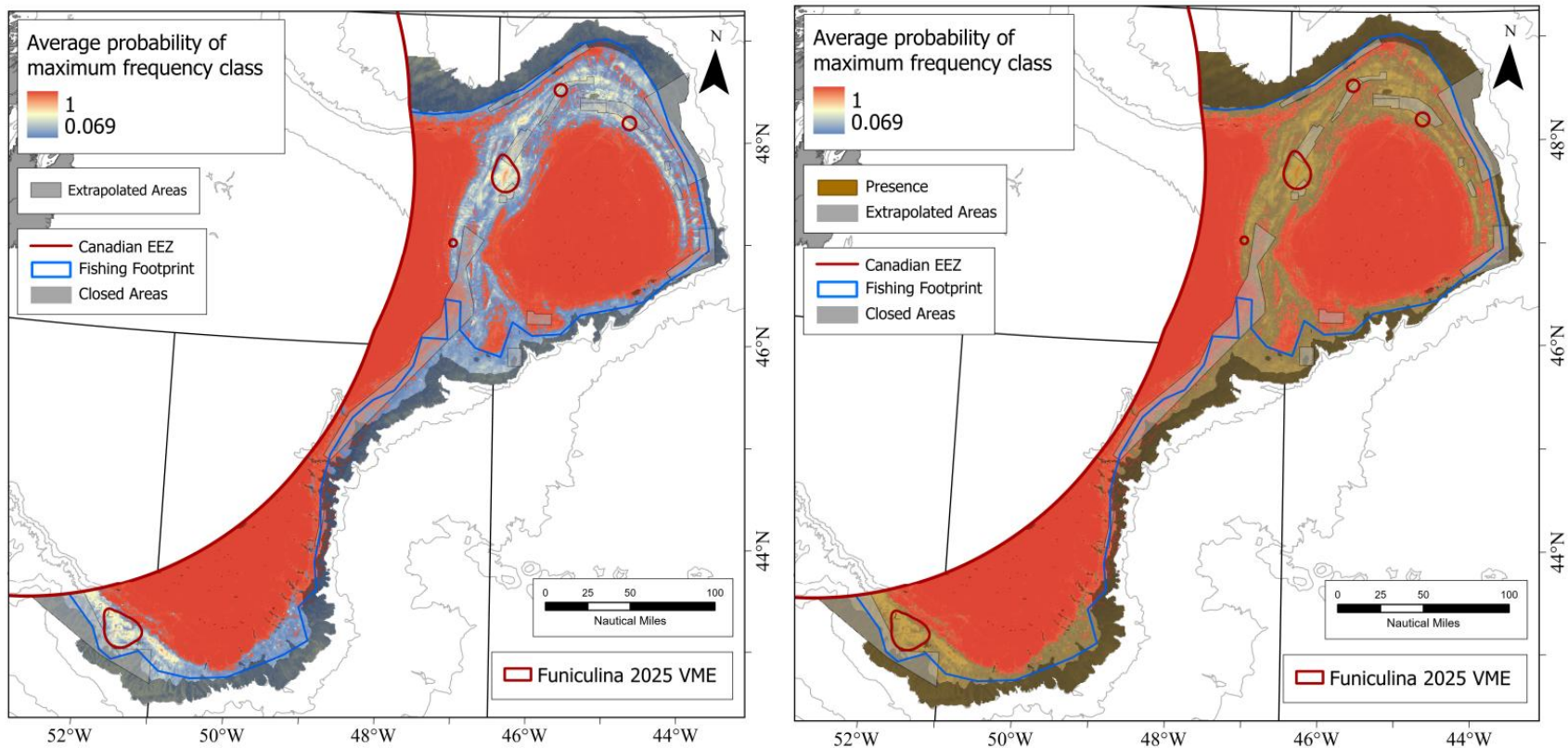
Figure 44. Left Panel. The 2025 Funiculina KDE VME polygons (Kenchington et al., 2025) superimposed on the average probability of the maximum frequency class (presence or absence) from 10 SDM runs for Funiculina (Murillo et al., 2024). Right Panel. The 2025 Funiculina KDE VME polygons (Kenchington et al., 2025) superimposed on the average probability of the maximum frequency class (presence or absence) from 10 SDM runs for Funiculina which itself is superimposed with a 30% transparent overlay showing areas where the SDM predicts presence for Funiculina created with a threshold optimised to ensure that resulting Sensitivity=Specificity (Murillo et al., 2024).
