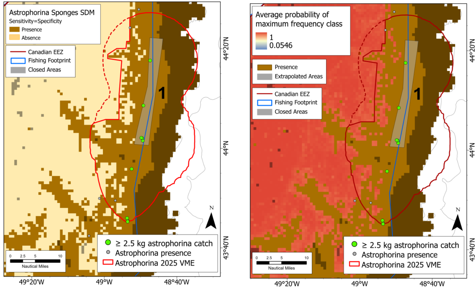
Figure 25. Area 1. Left Panel. Map of the proposed modification (solid red line) of the 2025 Astrophorina Sponge KDE VME polygon (red dashed lines) and showing the underlying SDM (brown area showing predicted presence of Astrophorina Sponges). Right Panel. Map of the proposed modification (solid red line) of the 2025 Astrophorina Sponge KDE VME polygon (red dashed lines) near Area 1 in relation to the average probability of the maximum frequency class for absence values from 10 SDM runs for the Astrophorina Sponges (Murillo et al., 2024). Closed areas are indicated in grey shading. Catches of \geq 2.5 kg, the threshold for the KDE analyses, and all other catches with < 2.5 kg are shown.
